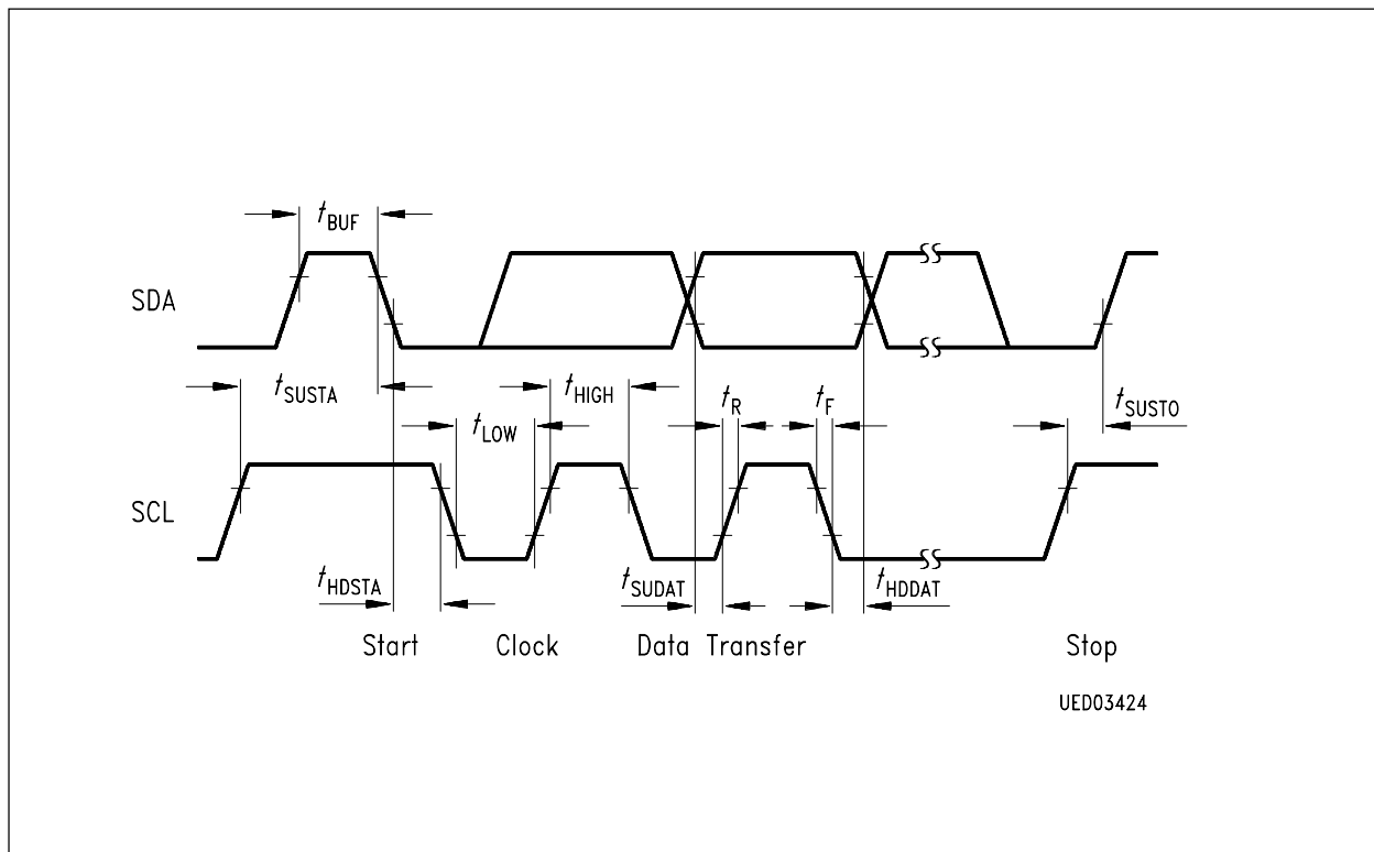
I²C Bus Timing Diagram
