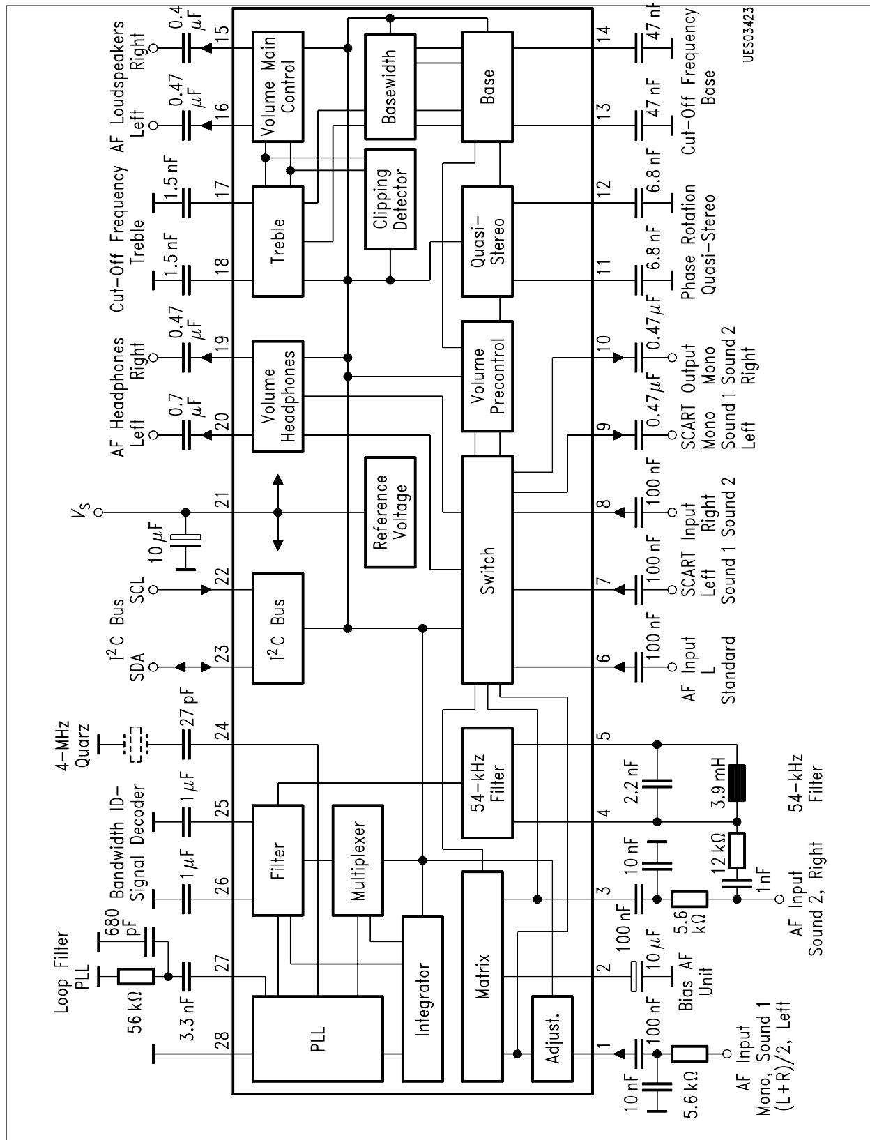
Application Circuit 3
