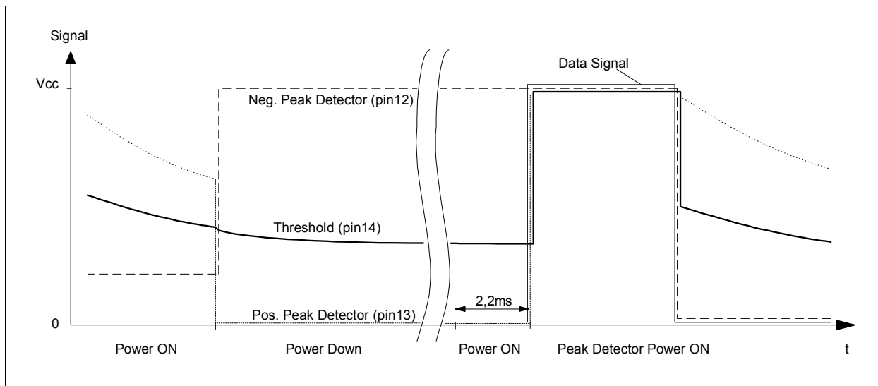
Figure 3-30 Power down mode
