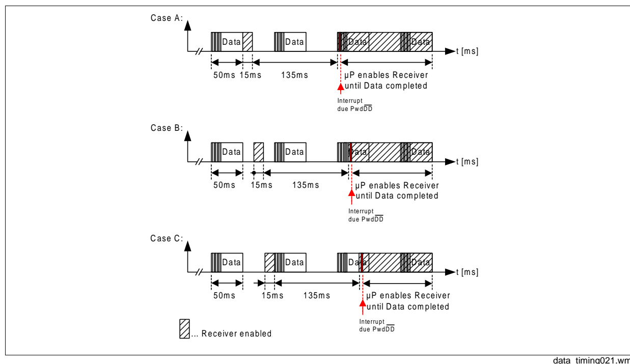
Figure 3-35 3 possible timings
