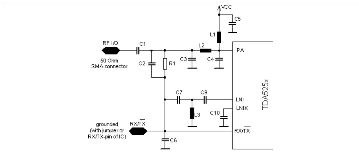
Figure 3-4 TX_Mode
