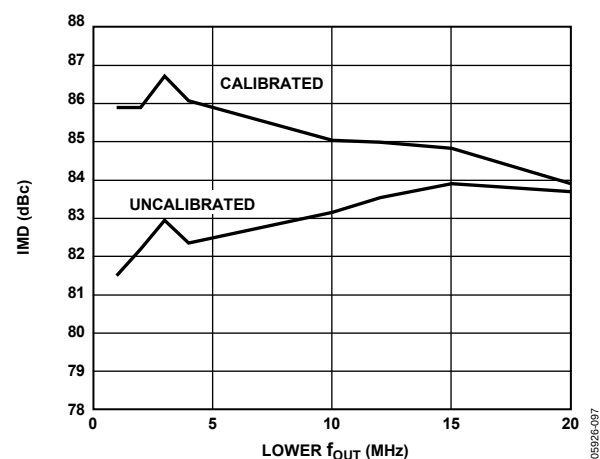
Figure 87. IMD vs. Lower f_{OUT} at 175 MSPS and I_{OUTFS} = 2\text{ mA}
