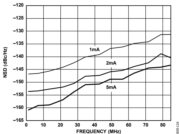
Figure 16. NSD vs. f_{OUT} and I_{OUTS} @ 175 MSPS
