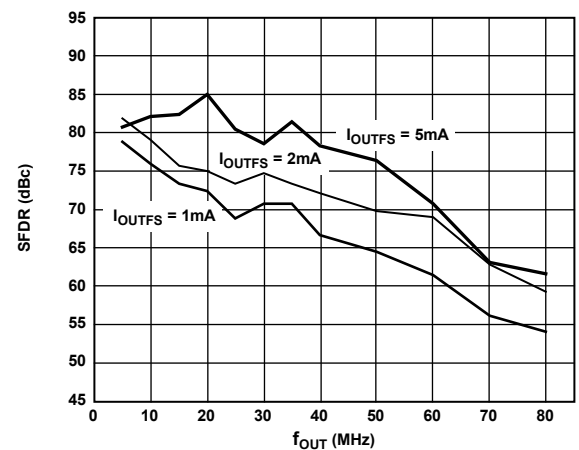
Figure 12. SFDR vs. f OUT and I OUTFS @ 175 MSPS
