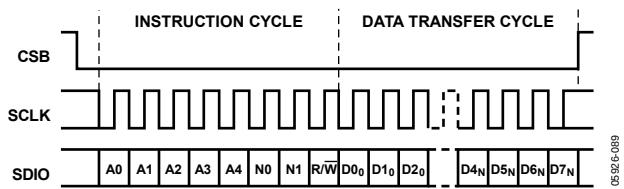
Figure 74. Serial Register Interface Timing, LSB First Write
