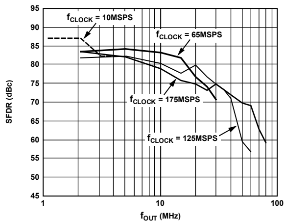
Figure 7. SFDR vs. f OUT
