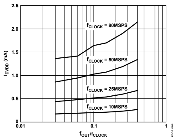
Figure 83. I_{DVDD} vs. f_{OUT}/f_{CLOCK} Ratio at DVDD = 1.8 V
