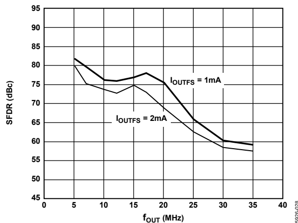
Figure 31. SFDR vs. f_{OUT} and I_{OUTFS} at 80 MS/SPS
