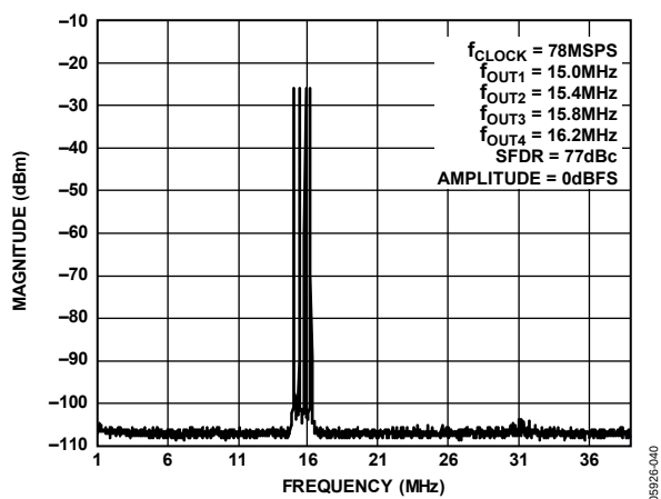
Figure 26. Four-Tone SFDR
