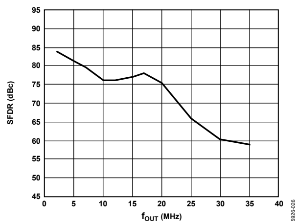
Figure 29. SFDR vs. f_{OUT} at 80 MS/SPS
