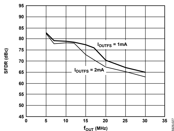
Figure 30. SFDR vs. f_{OUT} and I_{OUTFS} at 65 MS/SPS
