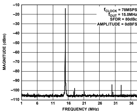
Figure 24. Single-Tone SFDR
