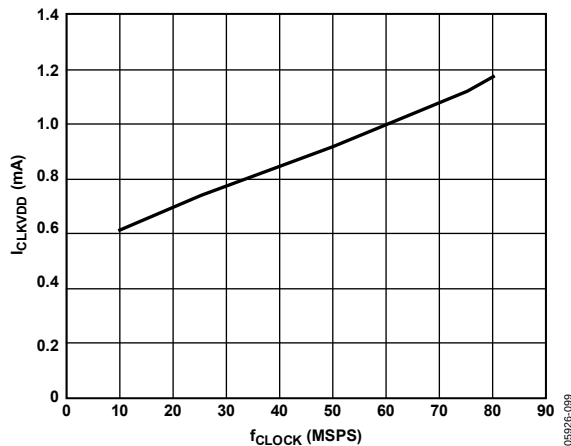
Figure 85. I_{CLKVDD} vs. f_{CLOCK} (Differential Clock Mode) at CLKVDD = 1.8\text{ V}
