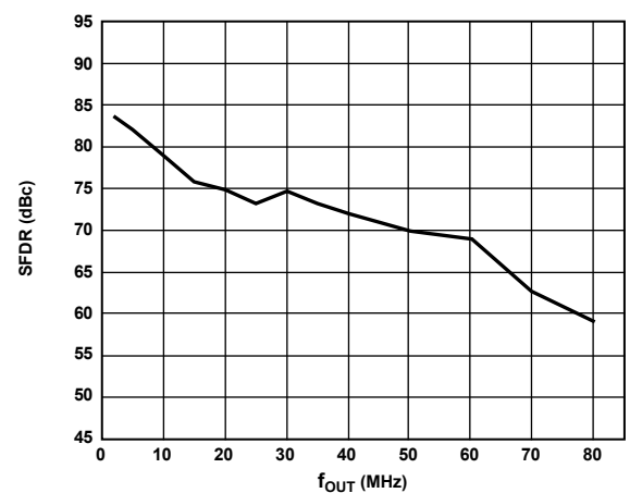
Figure 11. SFDR vs. f OUT @ 175 MSPS
