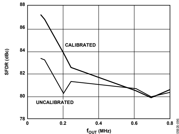
Figure 86. AD9707 SFDR vs. f_{OUT} at 175 MSPS and I_{OUTFS} = 2\text{ mA}
