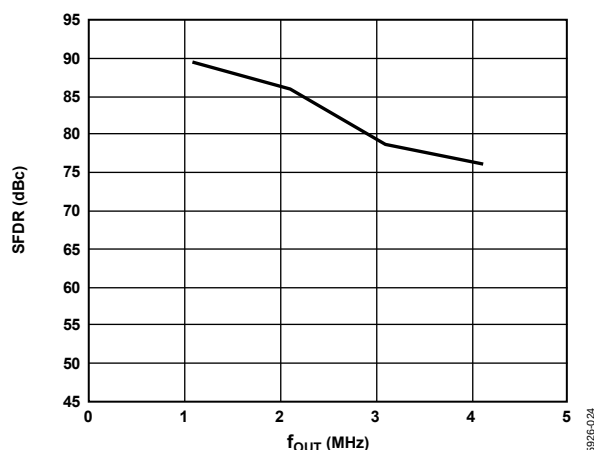
Figure 28. SFDR vs. f_{OUT} at 10 MS/SPS
