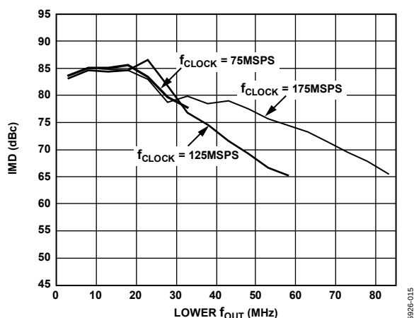
Figure 17. Dual-Tone IMD vs. Lower f_{OUT} and f_{CLOCK} @ 0 dBFS
