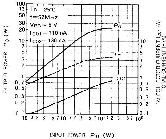
OUTPUT POWER, TOTAL CURRENT, 1st COLLECTOR CURRENT VS. INPUT POWER
