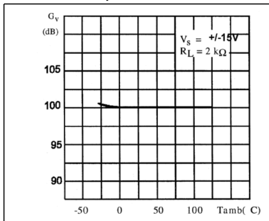
Figure 6. Output loop gain versus ambient temperature
