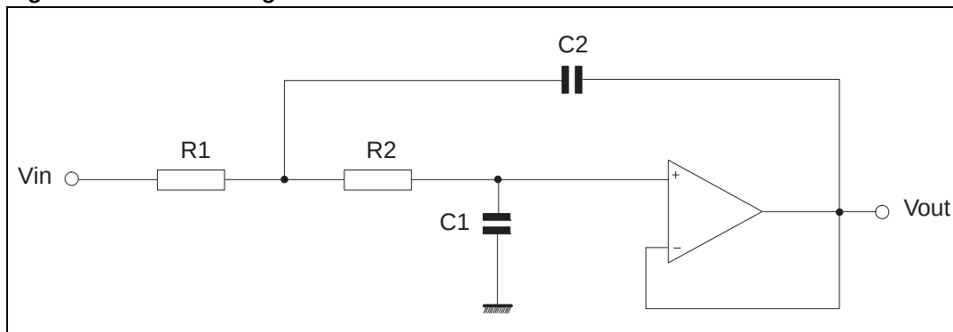
Figure 13. Filter configuration
