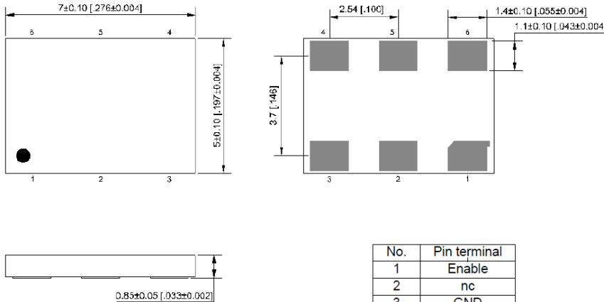
External Dimensions
