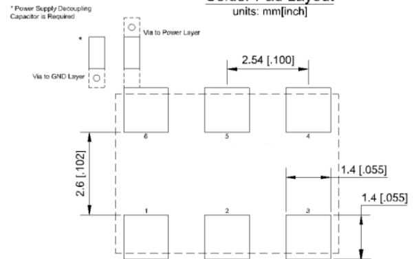
Recommended Solder Pad Layout units: mm[inch]
