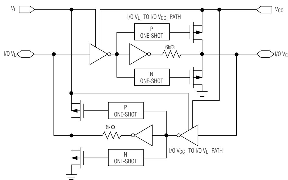
Figure 5. MAX3001E/MAX3002–MAX3012 Simplified Functional Diagram (1 I/O Line)
