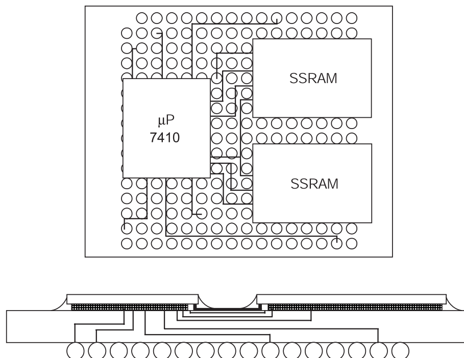
FIGURE 1 – MULTI-CHIP PACKAGE DIAGRAM
