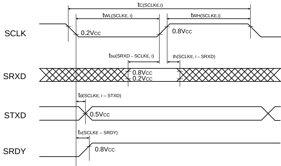
Fig. 82 Timing diagram (2)
