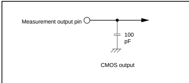
Fig. 79 Circuit for measuring output switching characteristics (1)
