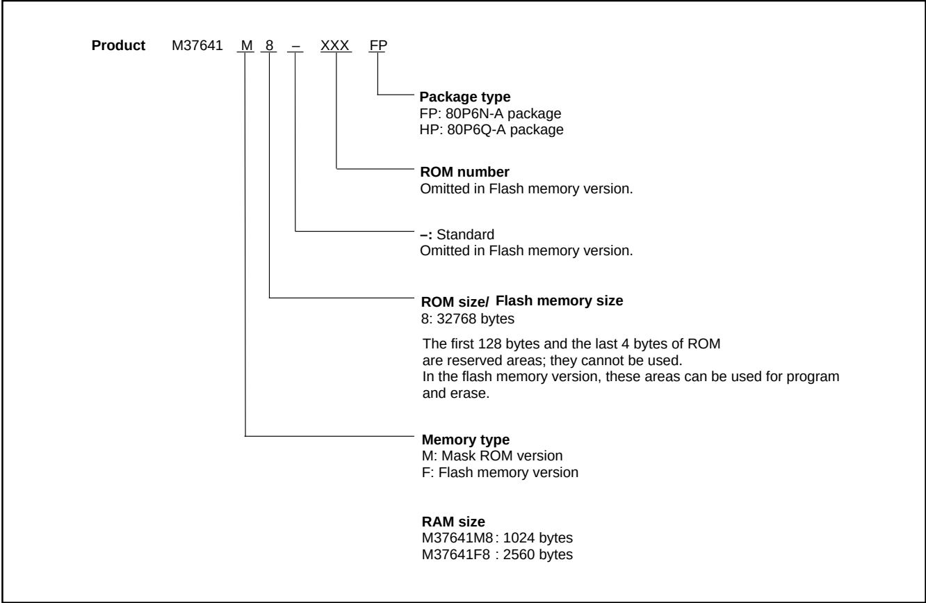
Fig. 4 Part numbering
