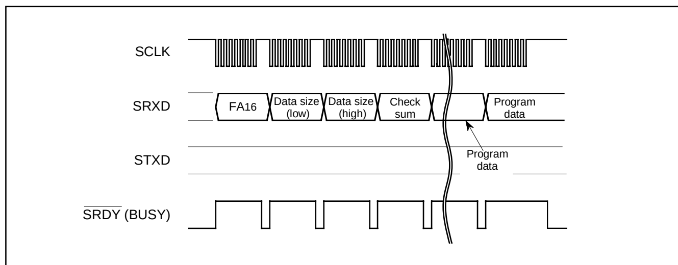
Fig. 104 Timing for download
