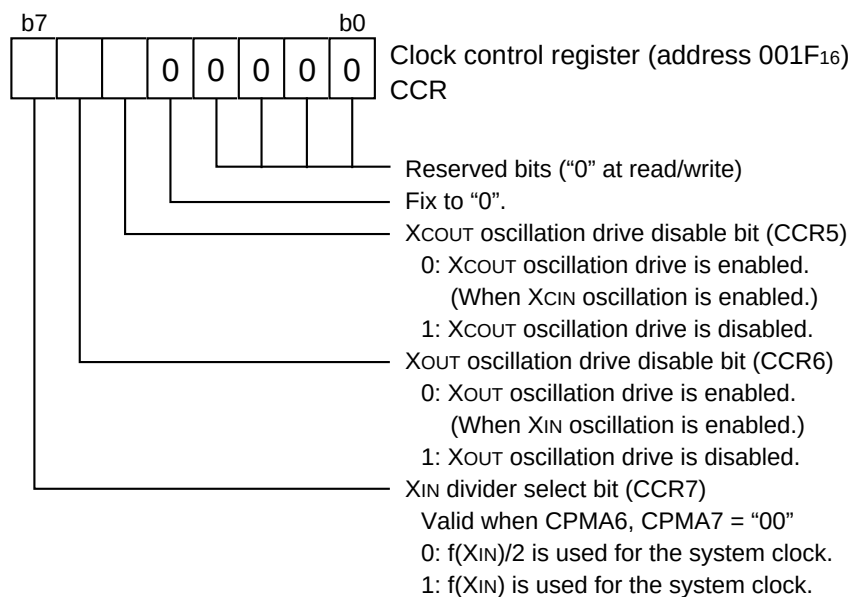
Fig. 66 Structure of clock control register
