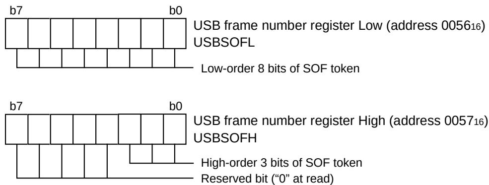
Fig. 44 Structure of USB frame number registers
