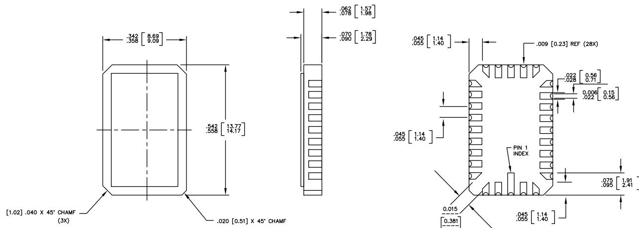
Figure 16. 28-Pad (350-Mil) LCC (001-51696)
