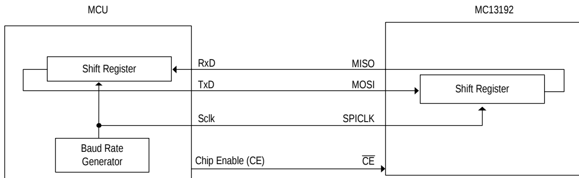
Figure 7. SPI Interface
