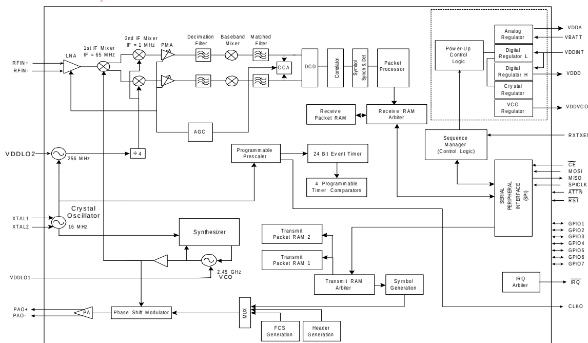
Figure 1. MC13192 Simplified Block Diagram
