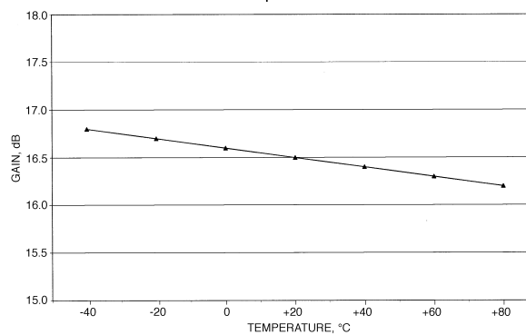
Gain vs Temperature at 900 MHz
