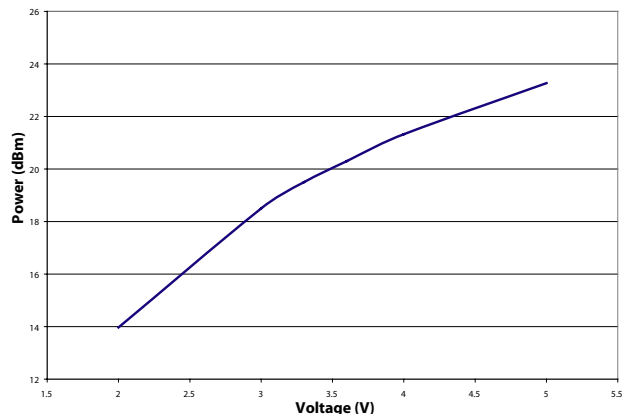
CMM6004-SC Evaluation board @ 900MHz OIP3 Over Voltage
