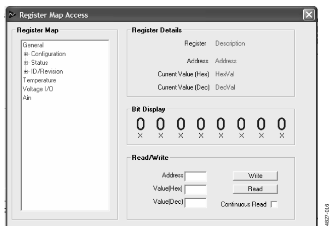
Figure 9. Register Map Access Window
