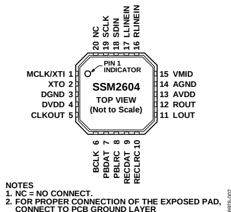
Figure 6. Pin Configuration
