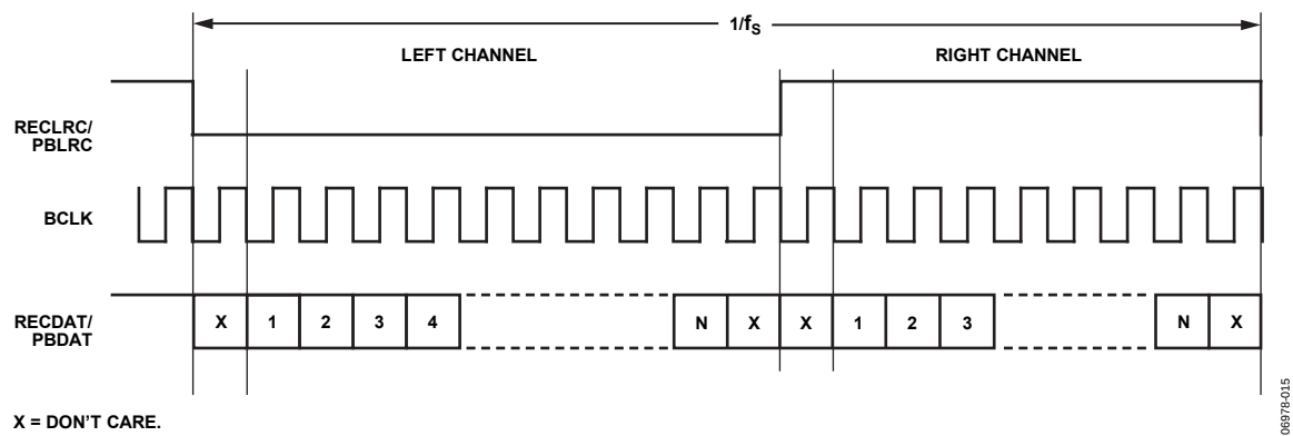
Figure 21. I²S Audio Input Mode
