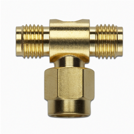
Model 72969 SMA T TYPE, JACK (F) / PLUG(M) / JACK (F)
