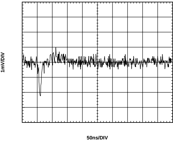
Figure 28. DAC-to-DAC Crosstalk
