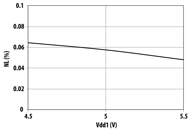
Figure 9. Non-Linearity vs Supply VDD1
