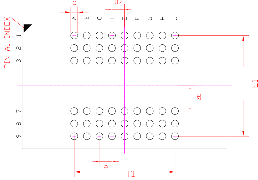
BOTTOM VIEW
