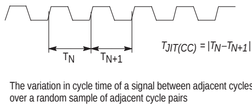
Figure 19. Cycle-to-Cycle Jitter
