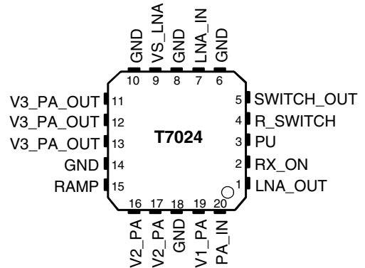
Figure 2-2. Pinning QFN20
