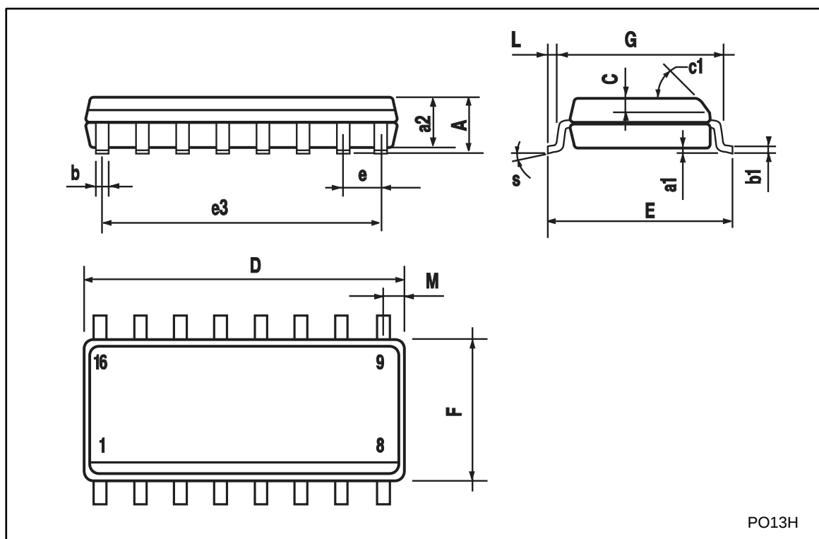
Figure 7: Plastic SO16 package mechanical outline
