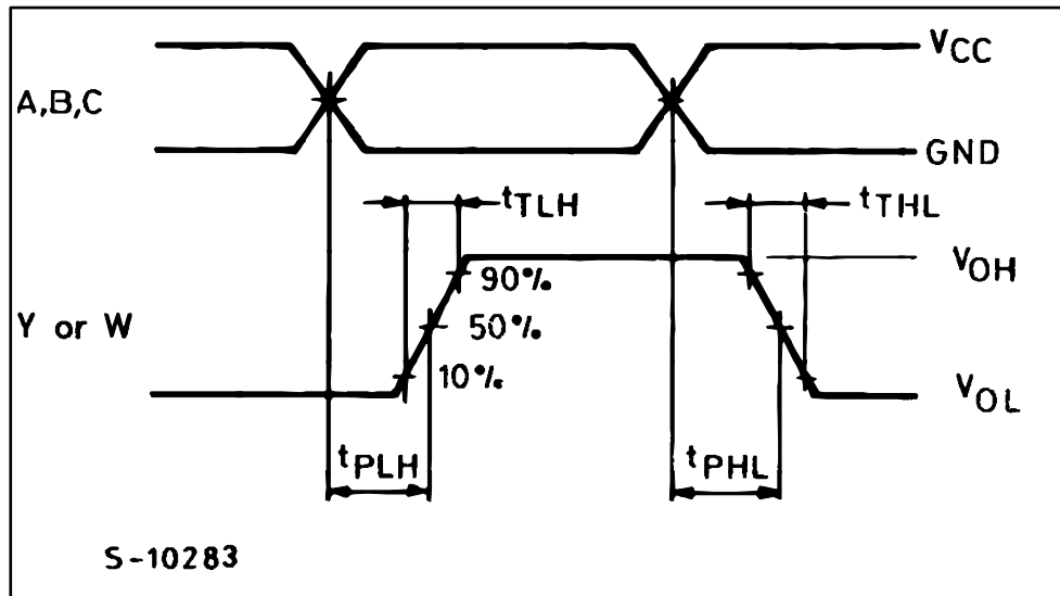
Figure 6: Waveform 2: propagation delay times ( f = 1 MHz; 50% duty cycle)
