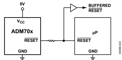
Figure 20. Bidirectional I-O \overline{\text{RESET}}
