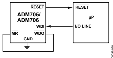
Figure 18. \overline{\text{RESET}} from WDO
