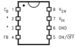
SO-8/DIP Package
