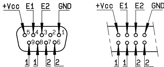
D-Sub connector
