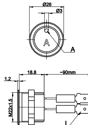
Point Illumination with Crimp Terminal male
