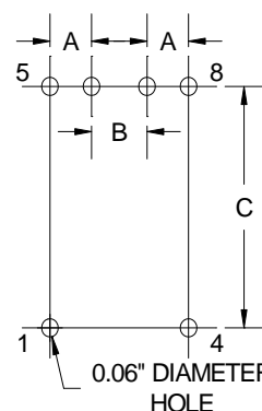
Board Layout
