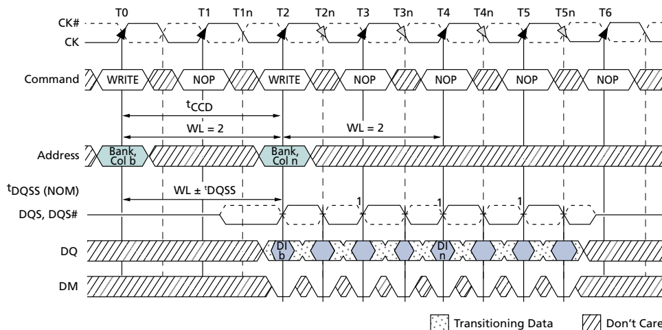
Figure 58: Consecutive WRITE-to-WRITE
