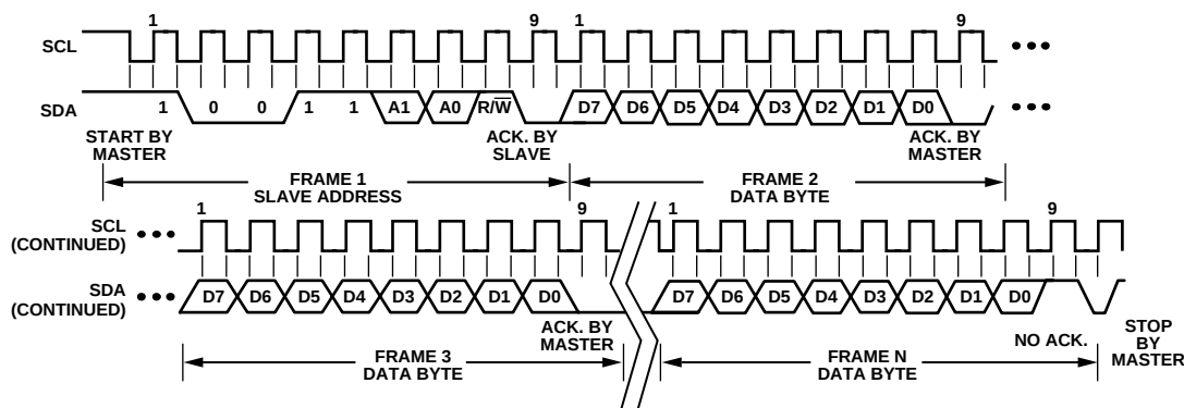
Figure 36. General SMBus Read Timing Diagram
