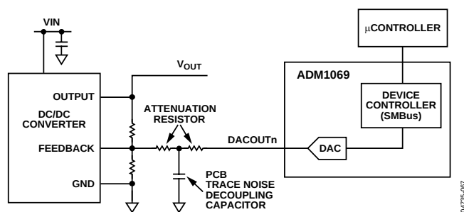
Figure 31. Open-Loop Margining System Using the ADM1069
