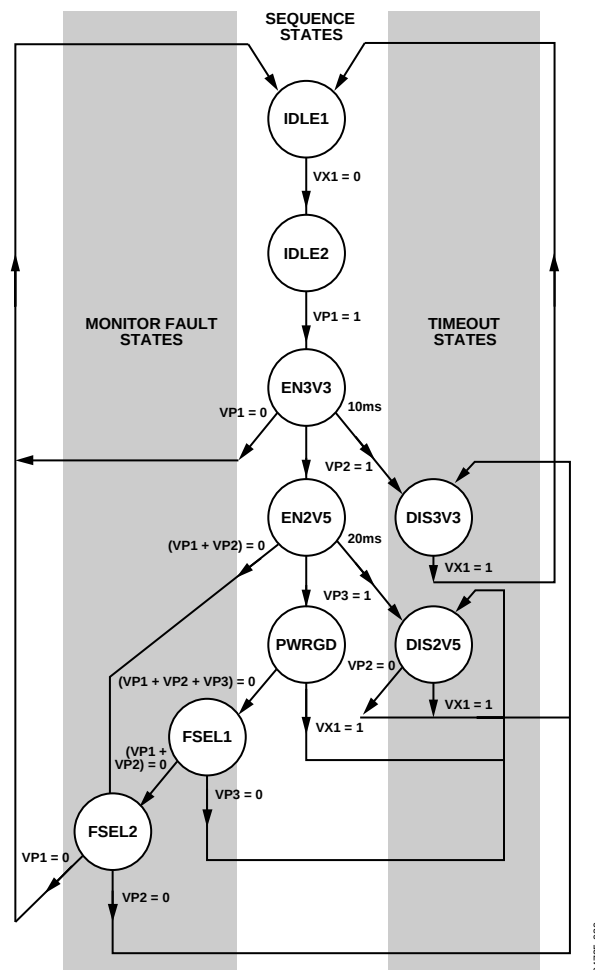
Figure 26. Sample Application Flow Diagram
