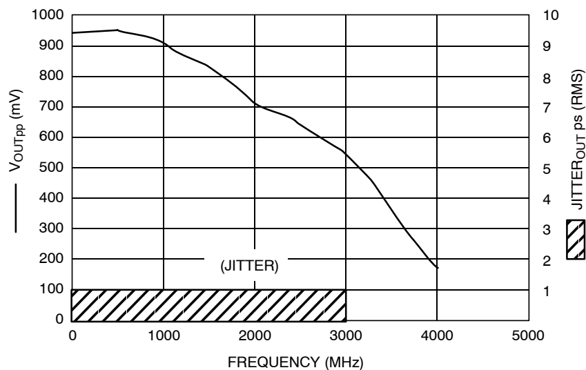
Figure 3. F_{\max}/\text{Jitter}
