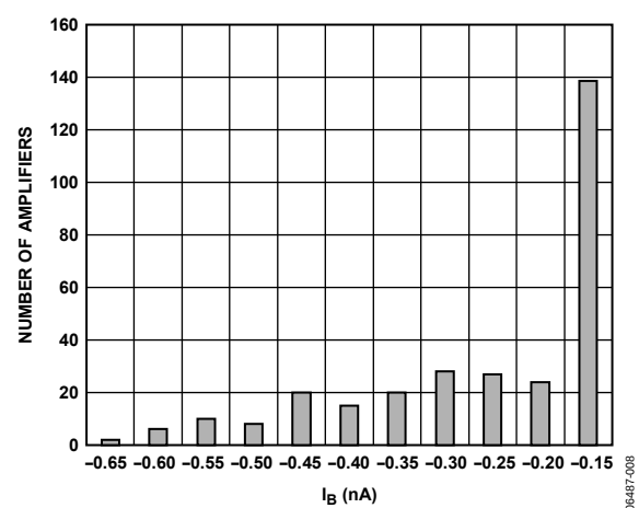
Figure 8. Input Bias Current, V_{SY} = \pm 5\text{ V}
