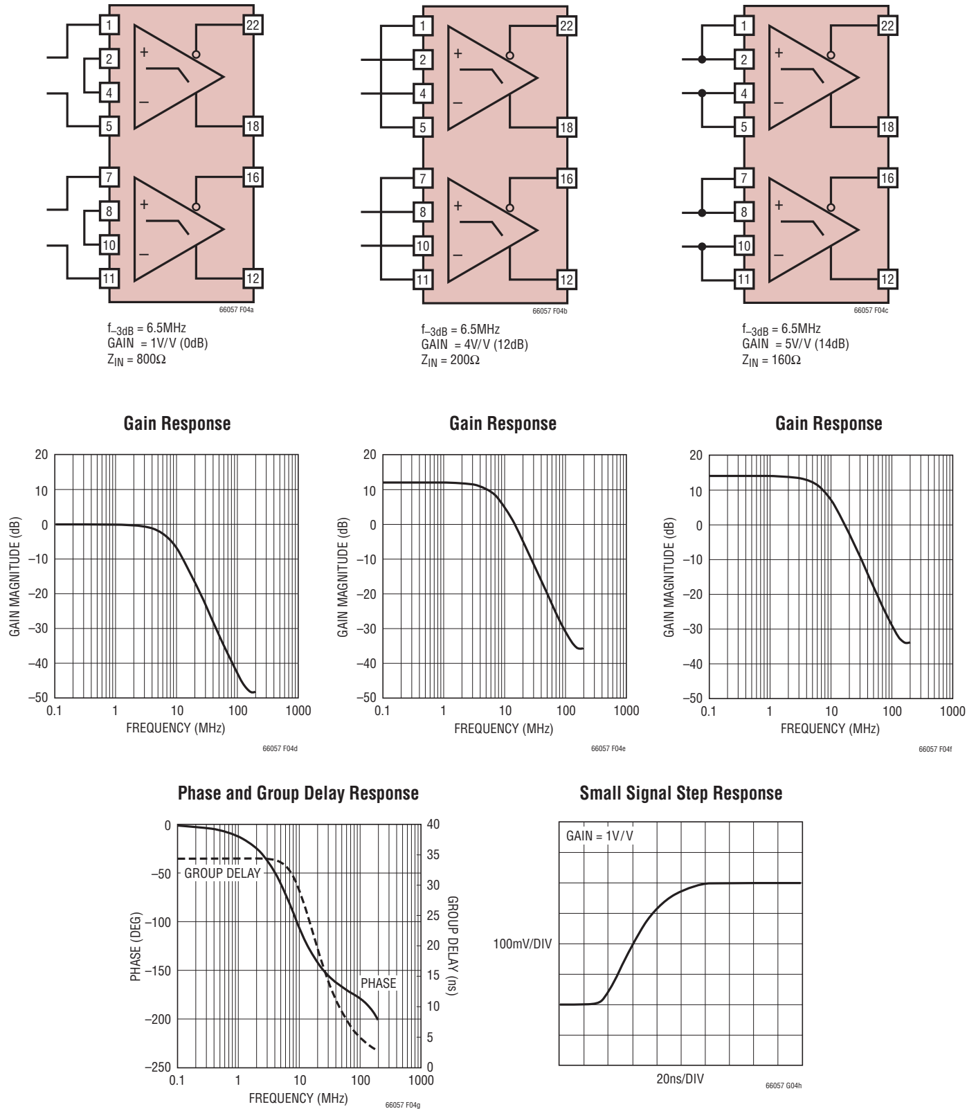
Figure 4. f_{-3dB} = 6.5\text{MHz} Filter Configurations without External Components
