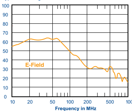
Typical shielding effectiveness in dB
