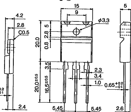
Outline Drawing ④8
