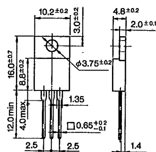
Outline Drawing ④9
