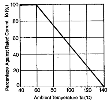
Io-Ta Deratings
