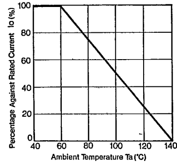
Io-Ta Deratings
