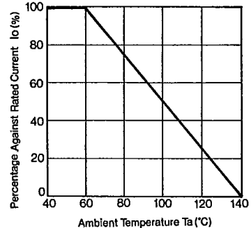
Io-Ta Deratings
