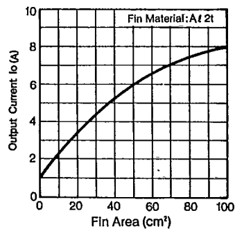
Io-Fin Characteristics
