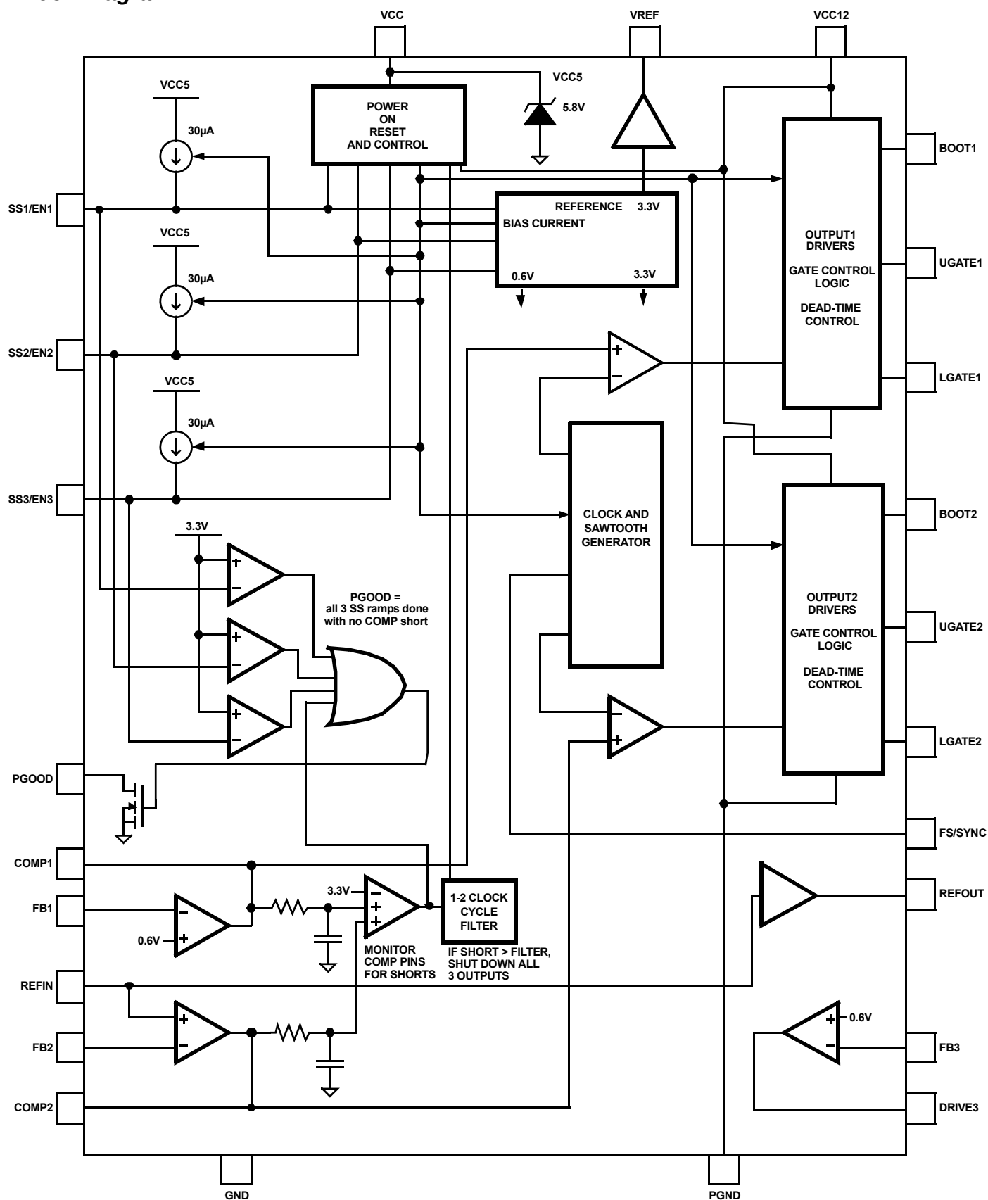
FIGURE 1. BLOCK DIAGRAM
