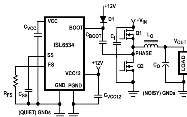
FIGURE 24. PRINTED CIRCUIT BOARD SMALL SIGNAL LAYOUT GUIDELINES
