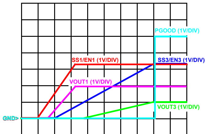
FIGURE 10. PGOOD OUTPUT
