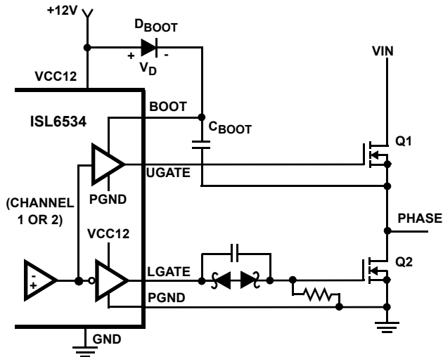
FIGURE 18. CAPACITIVE-COUPLED LGATE
