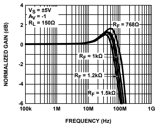
FIGURE 14. FREQUENCY RESPONSE FOR VARIOUS FEEDBACK RESISTORS, A V = -1
