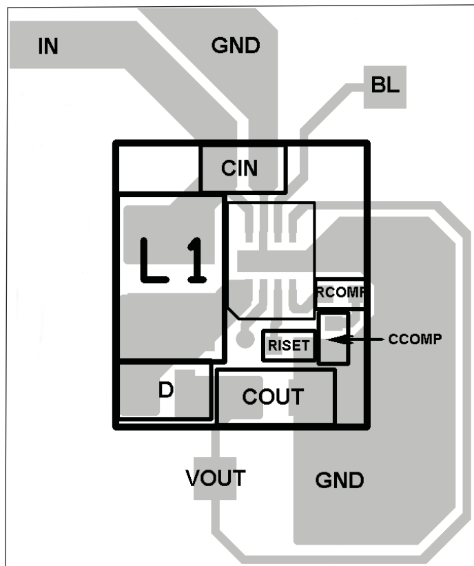
Figure 2– Layout
