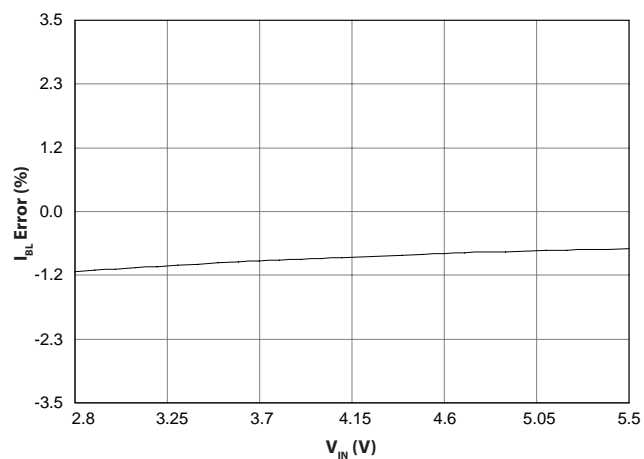
Normalized I_{BL} vs. Input Voltage
