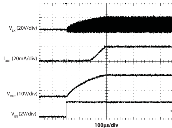
Start-Up Response
