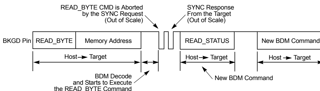
Figure 65. ACK Abort Procedure at the Command Level
