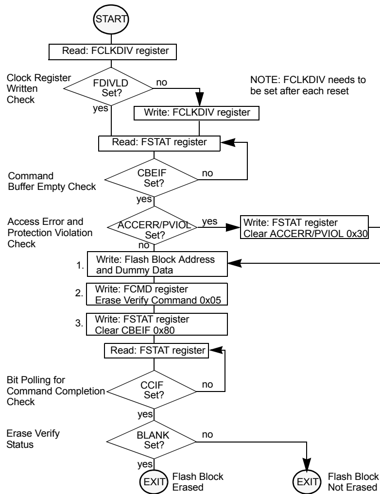
Figure 84. Example Erase Verify Command Flow
