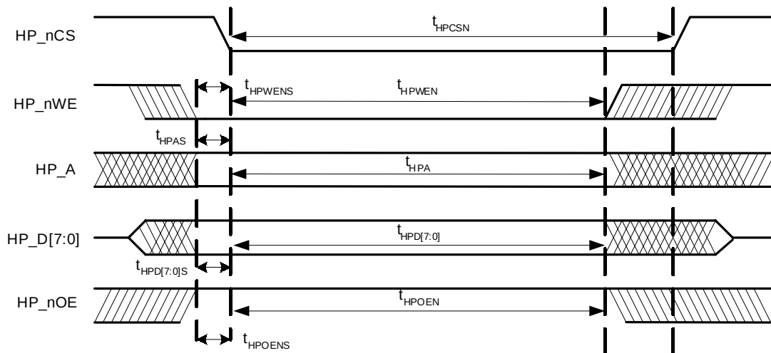
Figure 11. Host Parallel Write Cycle Timing
