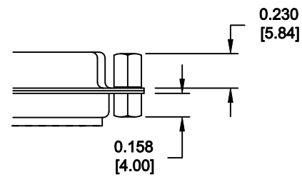
03X ..... 0.158" (BOARD SIDE) - 0.230" MATING SIDE
