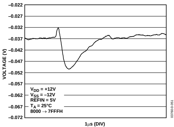
Figure 32. Major Code Transition Glitch Energy, \pm 12\text{V} Supplies
