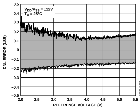
Figure 17. Differential Nonlinearity Error vs. Reference Voltage, ±12 V Supplies
