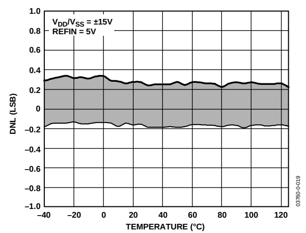
Figure 11. Differential Nonlinearity vs. Temperature, \pm 15\text{ V} Supplies
