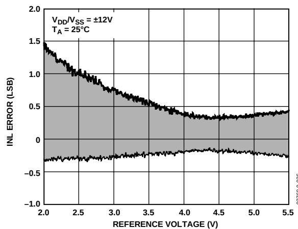
Figure 16. Integral Nonlinearity Error vs. Reference Voltage, ±12 V Supplies
