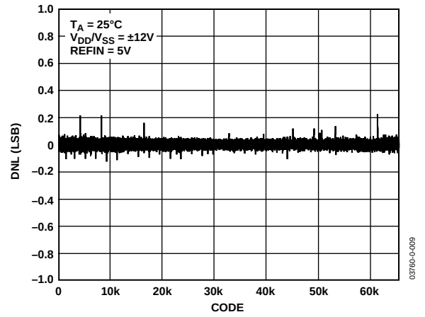
Figure 9. Differential Nonlinearity vs. Code, V_{DD}/V_{SS} = \pm 12\text{ V}
