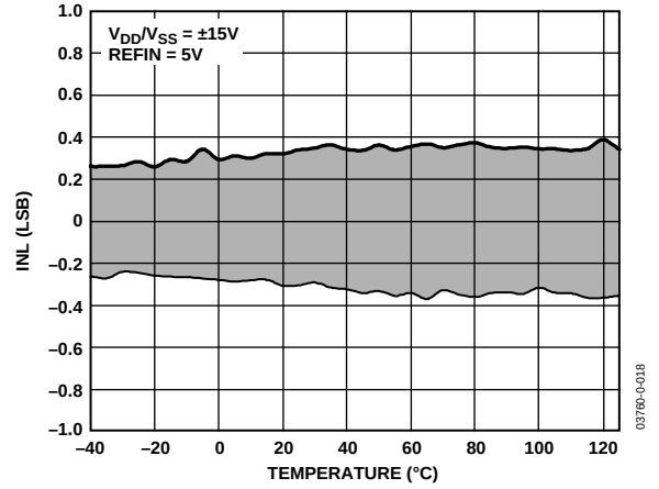
Figure 10. Integral Nonlinearity vs. Temperature, \pm 15\text{ V} Supplies
