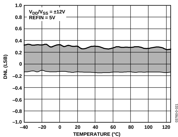
Figure 13. Differential Nonlinearity vs. Temperature, ±12 V Supplies
