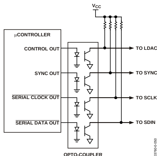
Figure 40. Opto-Isolated Interface
