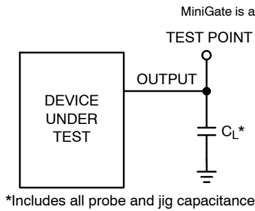
Figure 5. Test Circuit
