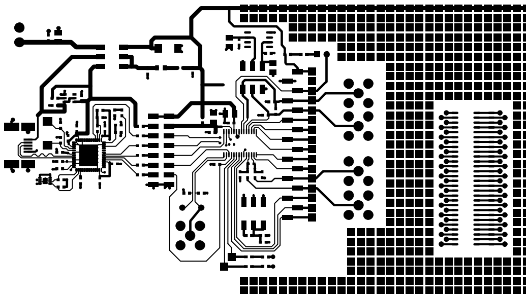
Figure 15. EVAL-AD7193EBZ Component Side View
