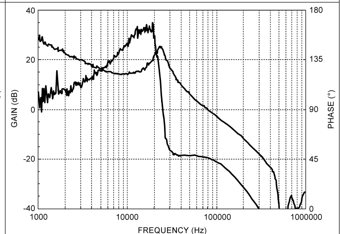
Figure 37. LM2854 500-kHz Bode Plot V_{IN} = 5\text{ V} , V_{OUT} = 3.3\text{ V} , I_{OUT} = 4\text{ A} R_{FB1} = 250\text{ k}\Omega , R_{COMP} = 1\text{ k}\Omega , C_{COMP} = 33\text{ pF} , L_{OUT} = 1.5\text{ }\mu\text{H} , C_{OUT} = 100\text{-}\mu\text{F Ceramic}
