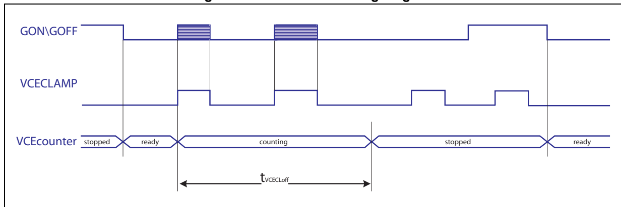
Figure 14. VCECLAMP timing diagram
