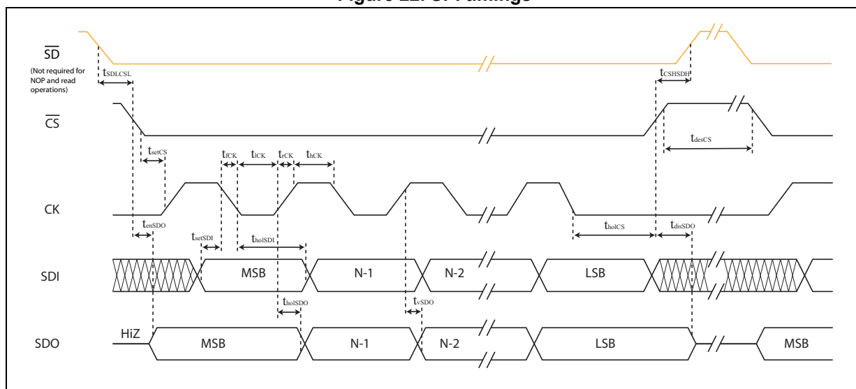
Figure 22. SPI timings
