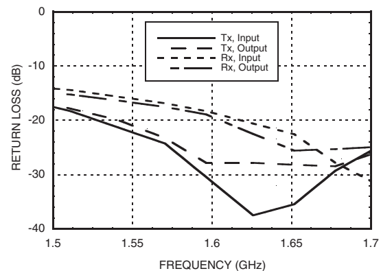
Return Loss with 1600 MHz Tuning
