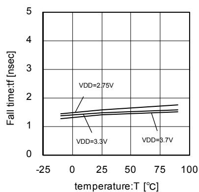
Fig.86 78MHz Fall-time temperature characteristics
