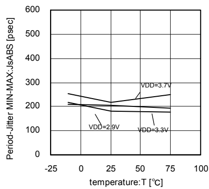
Fig.43 27MHz Jitter-MinMax temperature characteristics
