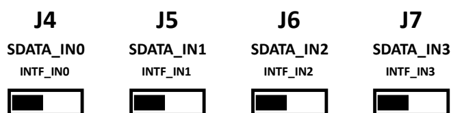
Figure 11. Input Routing Jumpers - I 2 S/TDM Configuration
