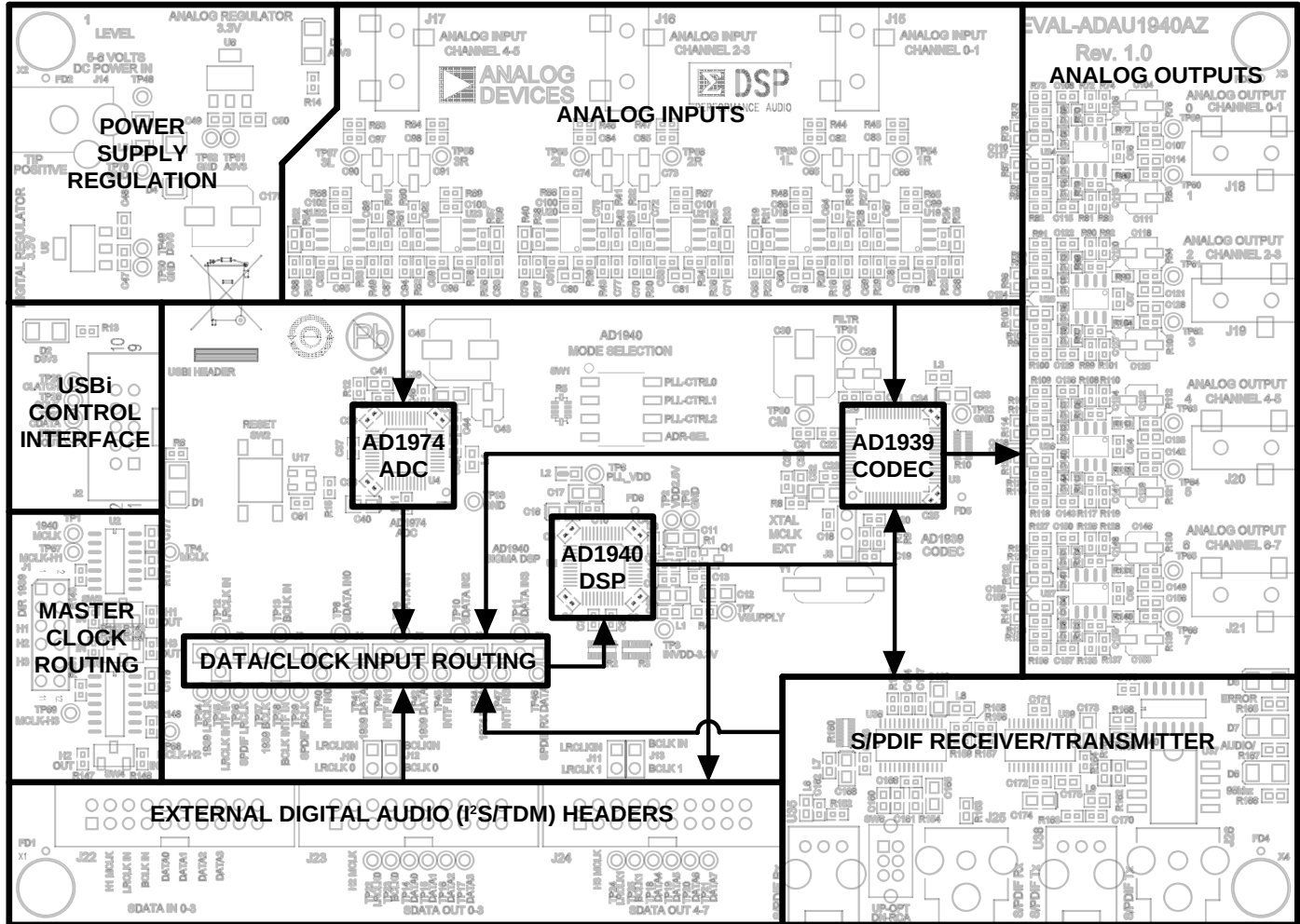
Figure 2. Board Layout Block Diagram
