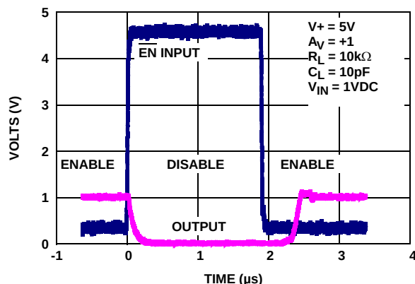
FIGURE 16. ENABLE/DISABLE TIMING
