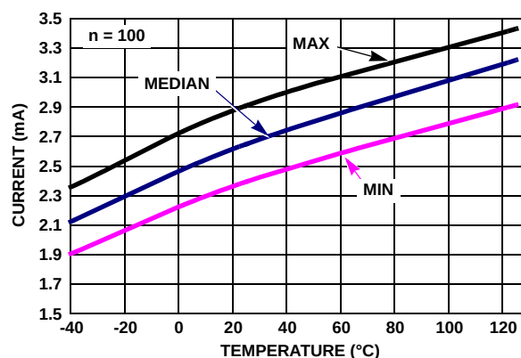
FIGURE 20. SUPPLY CURRENT vs TEMPERATURE, V_S = \pm 2.5V ENABLED, R_L = \text{INF}
