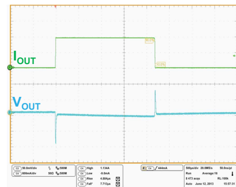
Figure 27. Load transient
