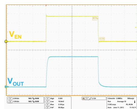
Figure 29. Turn-on time
