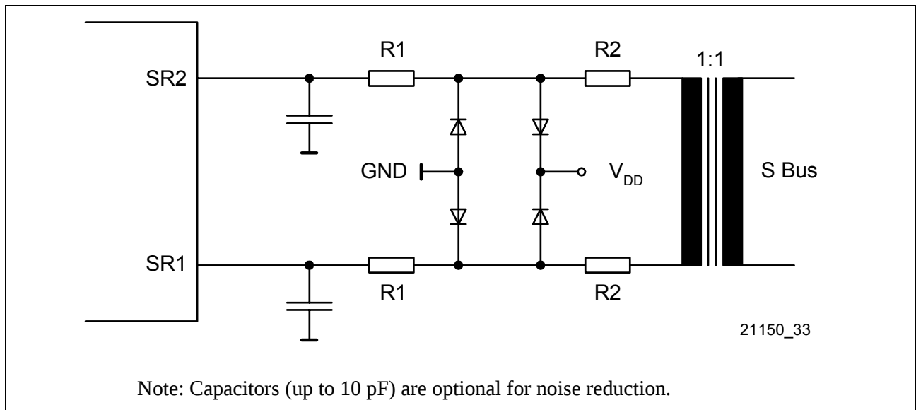
Figure 31 External Circuitry for Symmetrical Receivers
