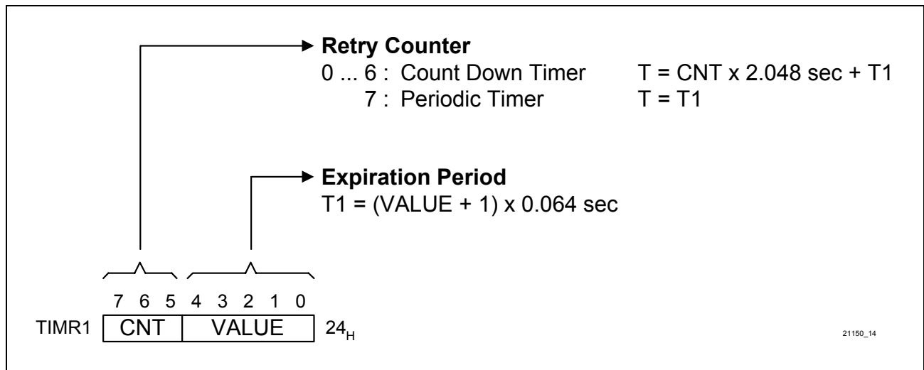
Figure 11 Timer 1 Register
