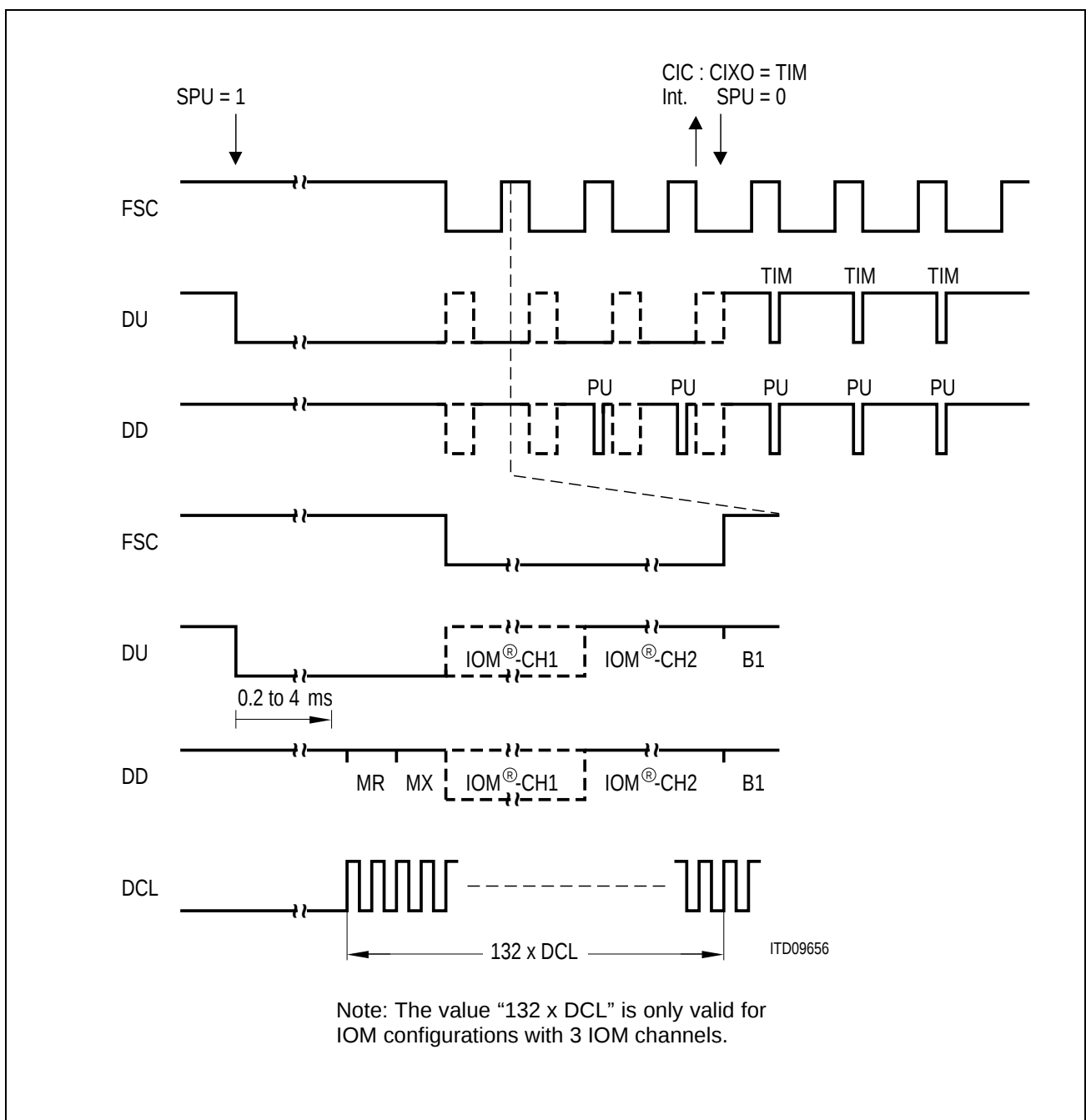
Figure 71 Activation of the IOM-2 interface
