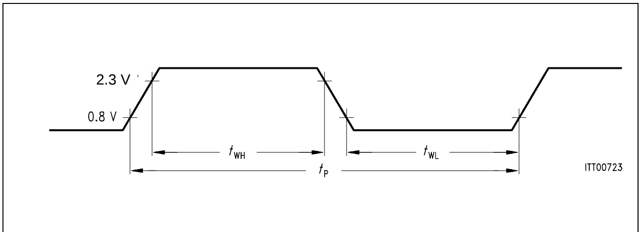
Figure 86 Definition of Clock Period and Width
