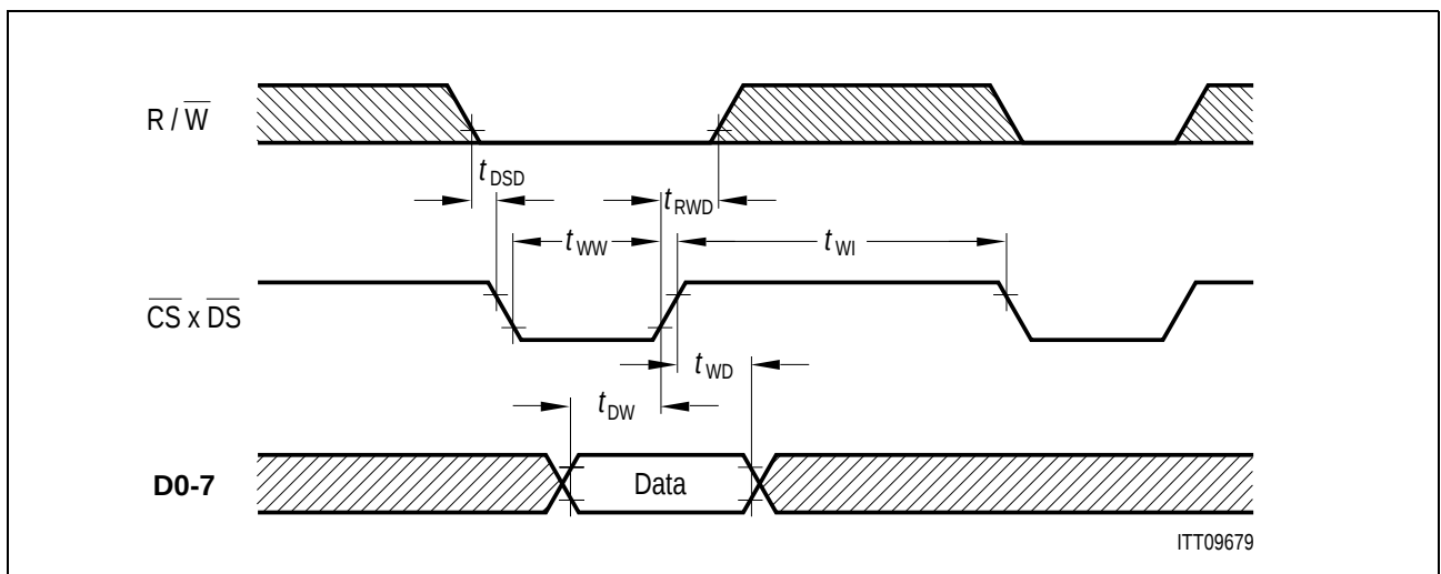
Figure 93 Microprocessor Write Cycle
