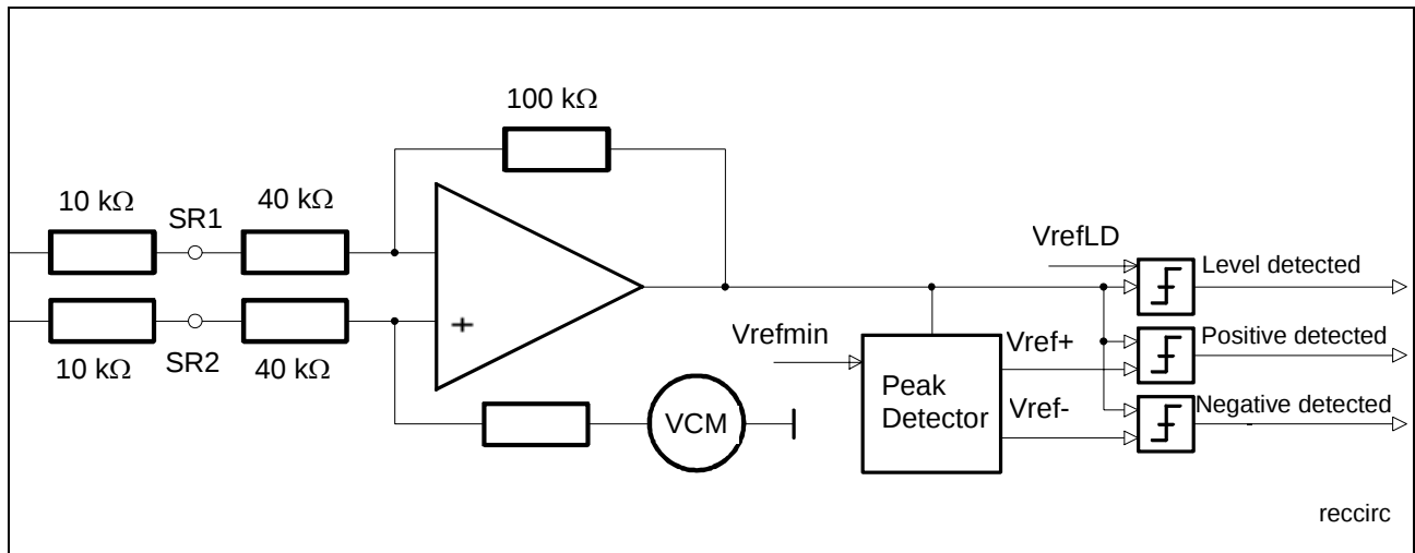
Figure 27 Equivalent Internal Circuit of the Receiver Stage
