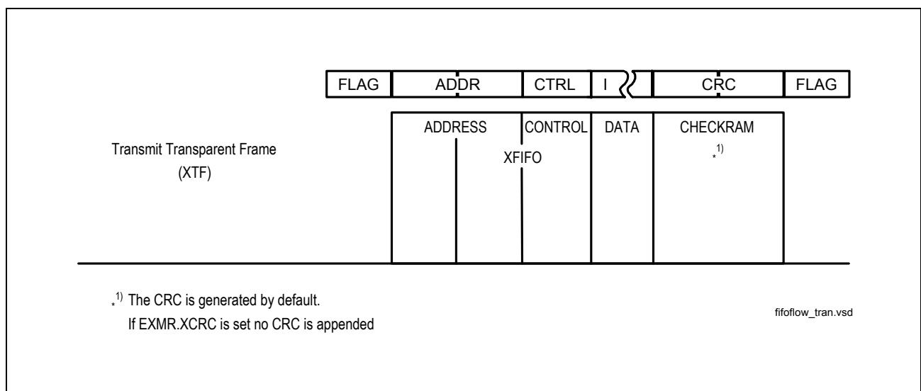
Figure 78 Transmit Data Flow
