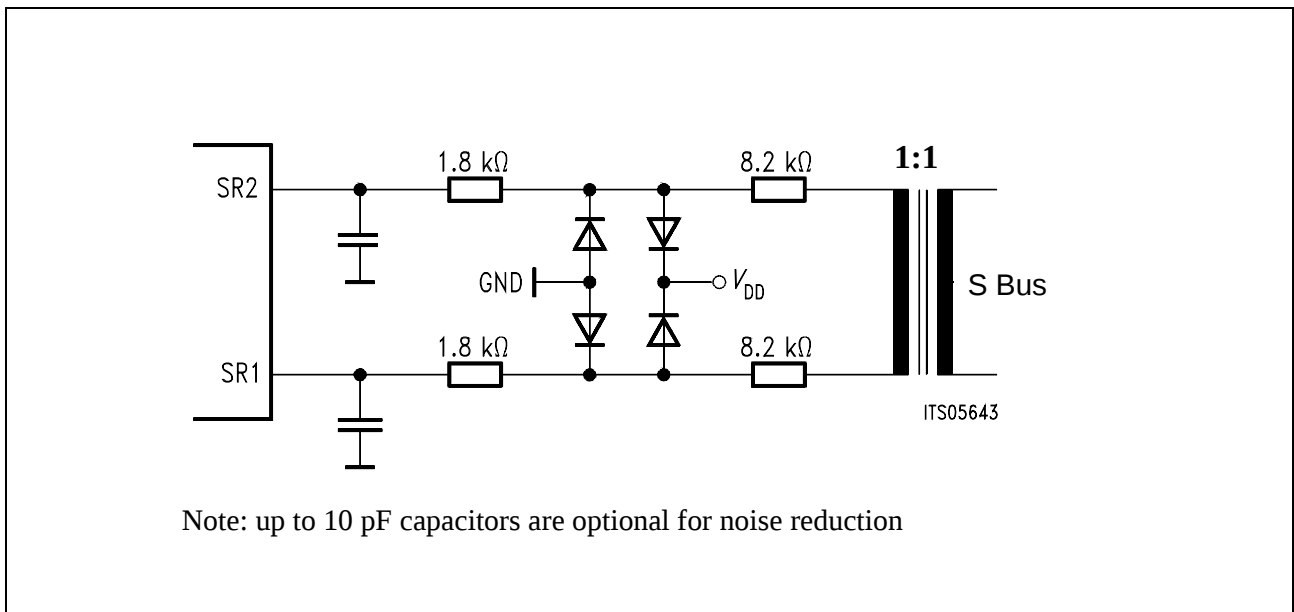
Figure 30 External Circuitry for Symmetrical Receivers
