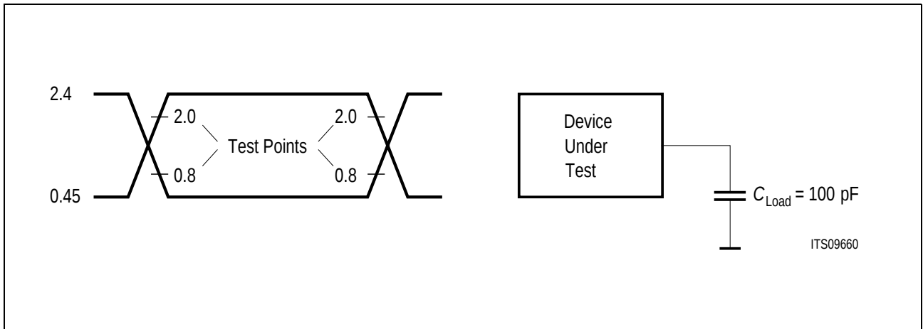
Figure 83 Input/Output Waveform for AC Tests
