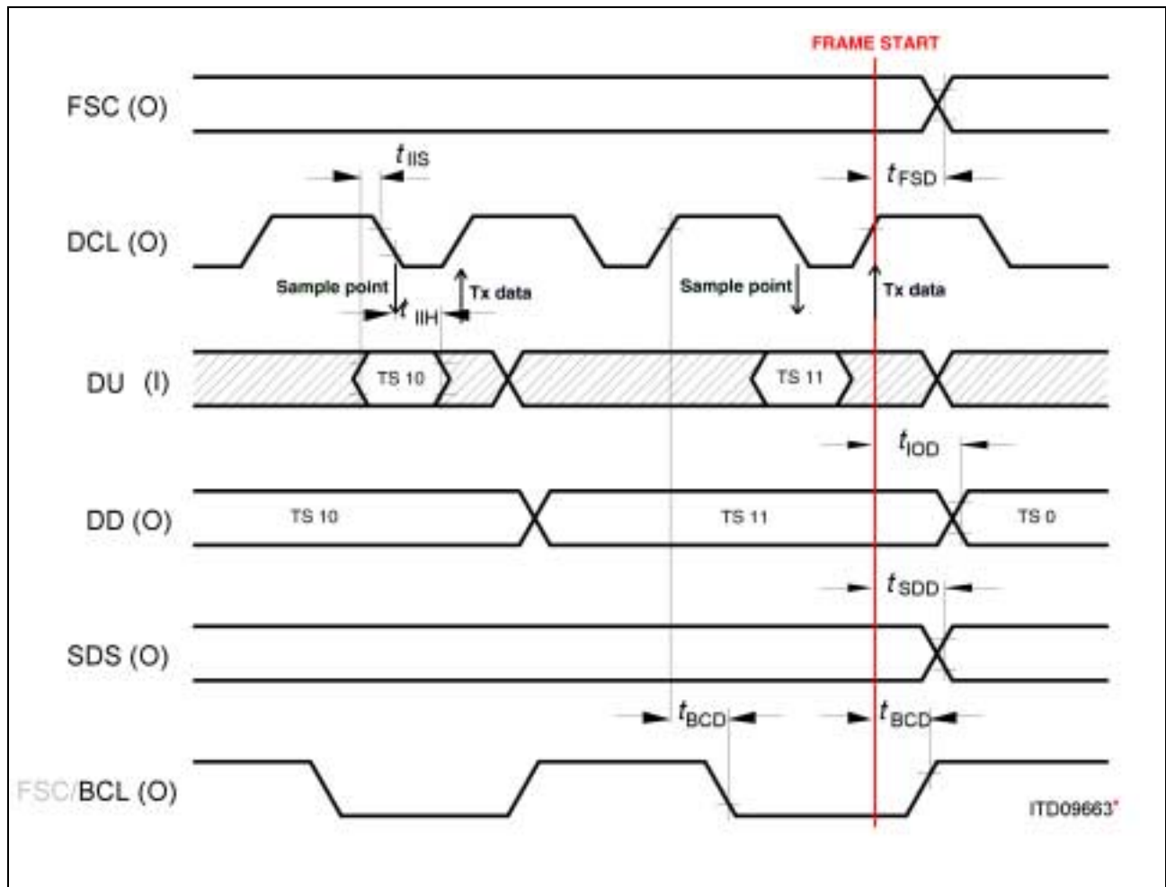
Figure 84 IOM-2 Timing (TE mode)
