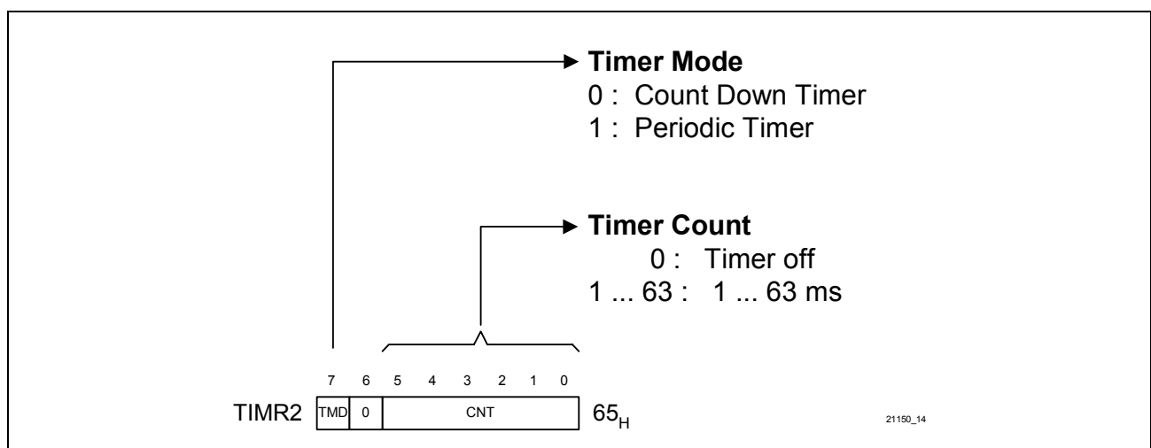
Figure 12 Timer 2 Register
