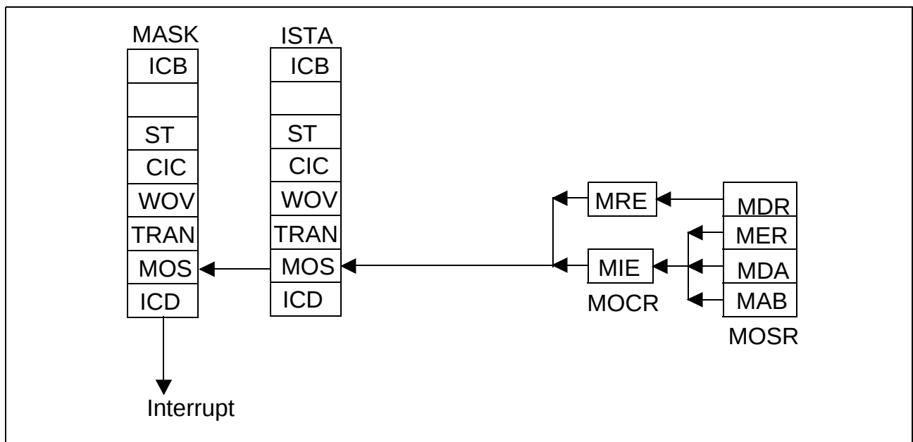
Figure 63 MONITOR Interrupt Structure
