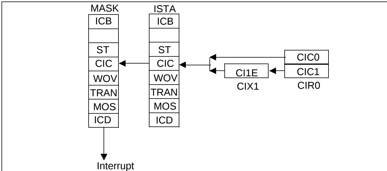
Figure 64 CIC Interrupt Structure
