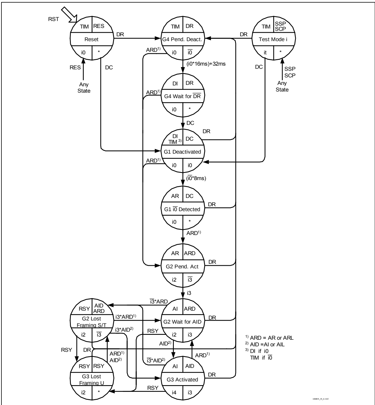
Figure 42 State Transition Diagram (NT)
