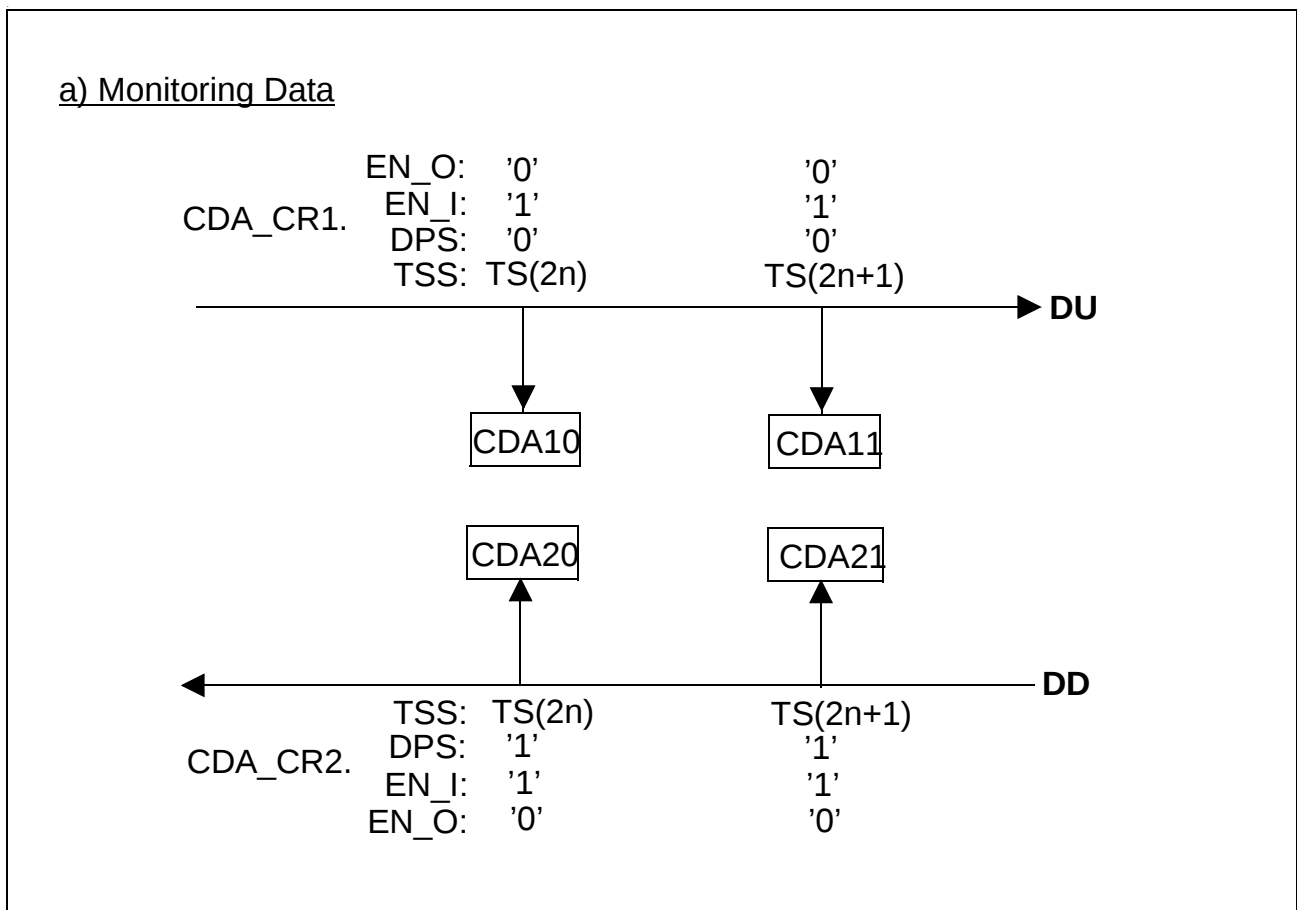
Figure 53 Example for Monitoring Data
