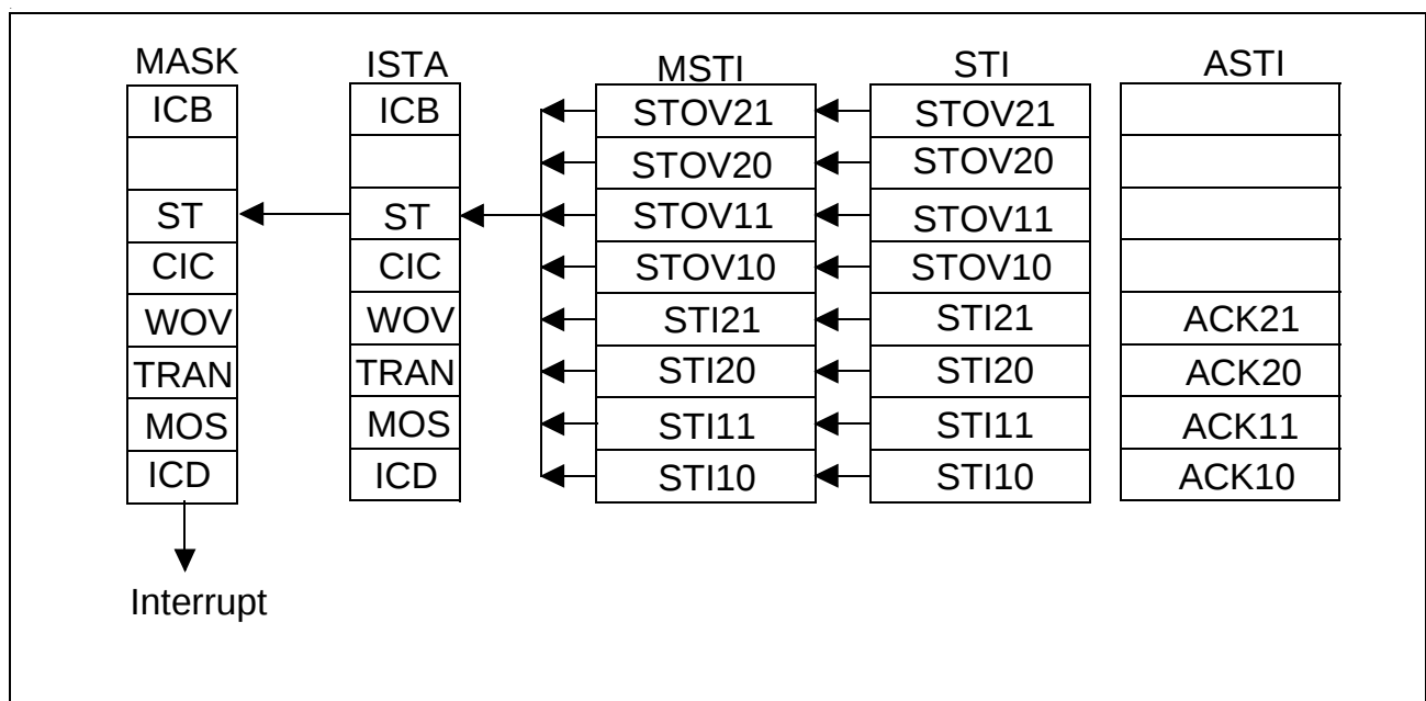
Figure 54 Interrupt Structure of the Synchronous Data Transfer
