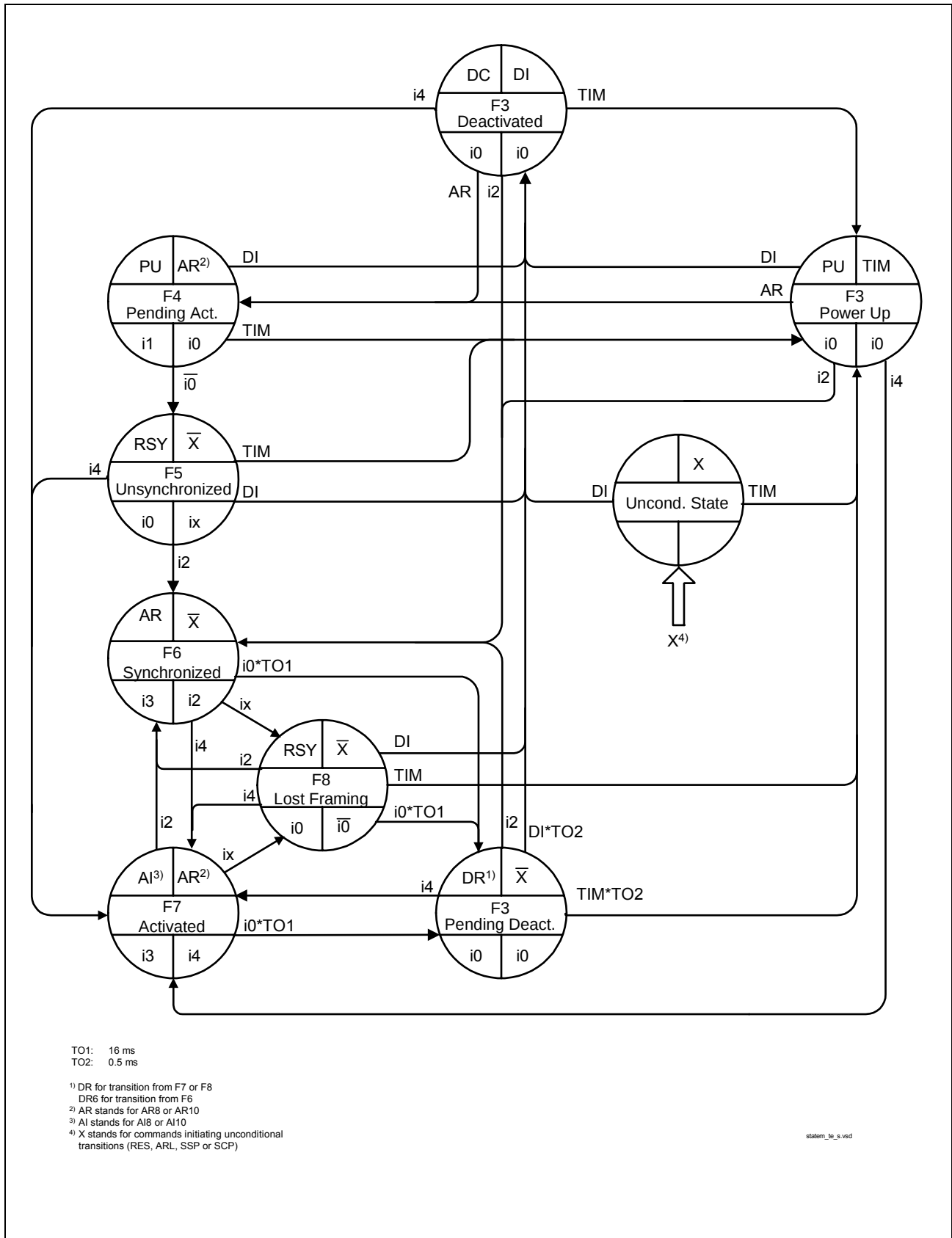
Figure 39 State Transition Diagram (TE, LT-T)
