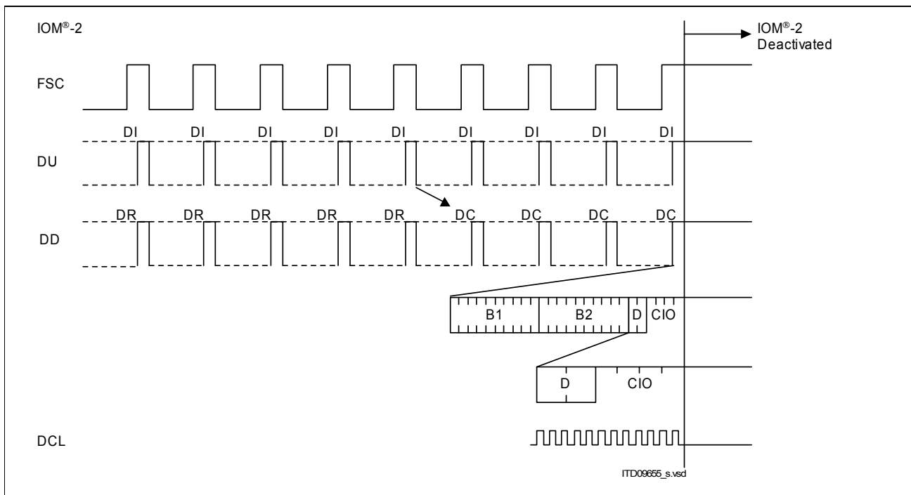
Figure 70 Deactivation of the IOM-2 Interface
