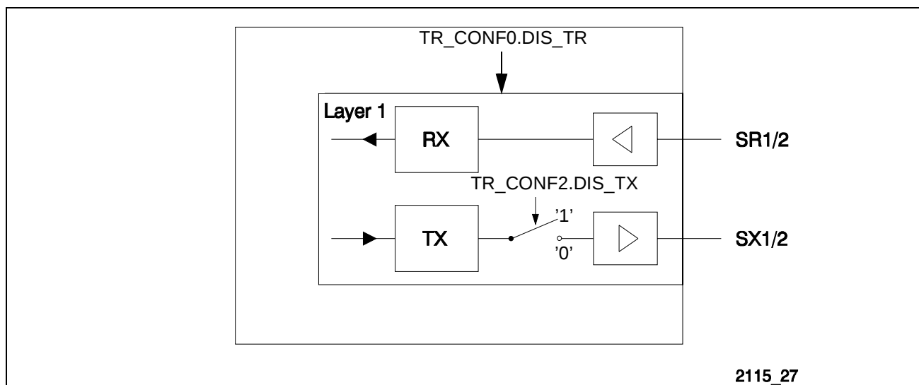
Figure 32 Disabling of S/T Transmitter
