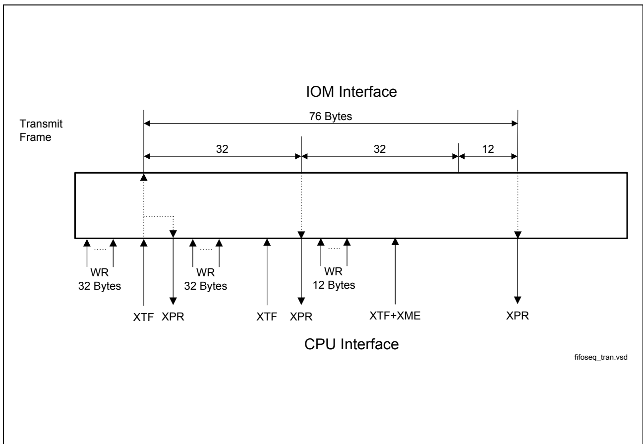
Figure 77 Transmission Sequence Example
