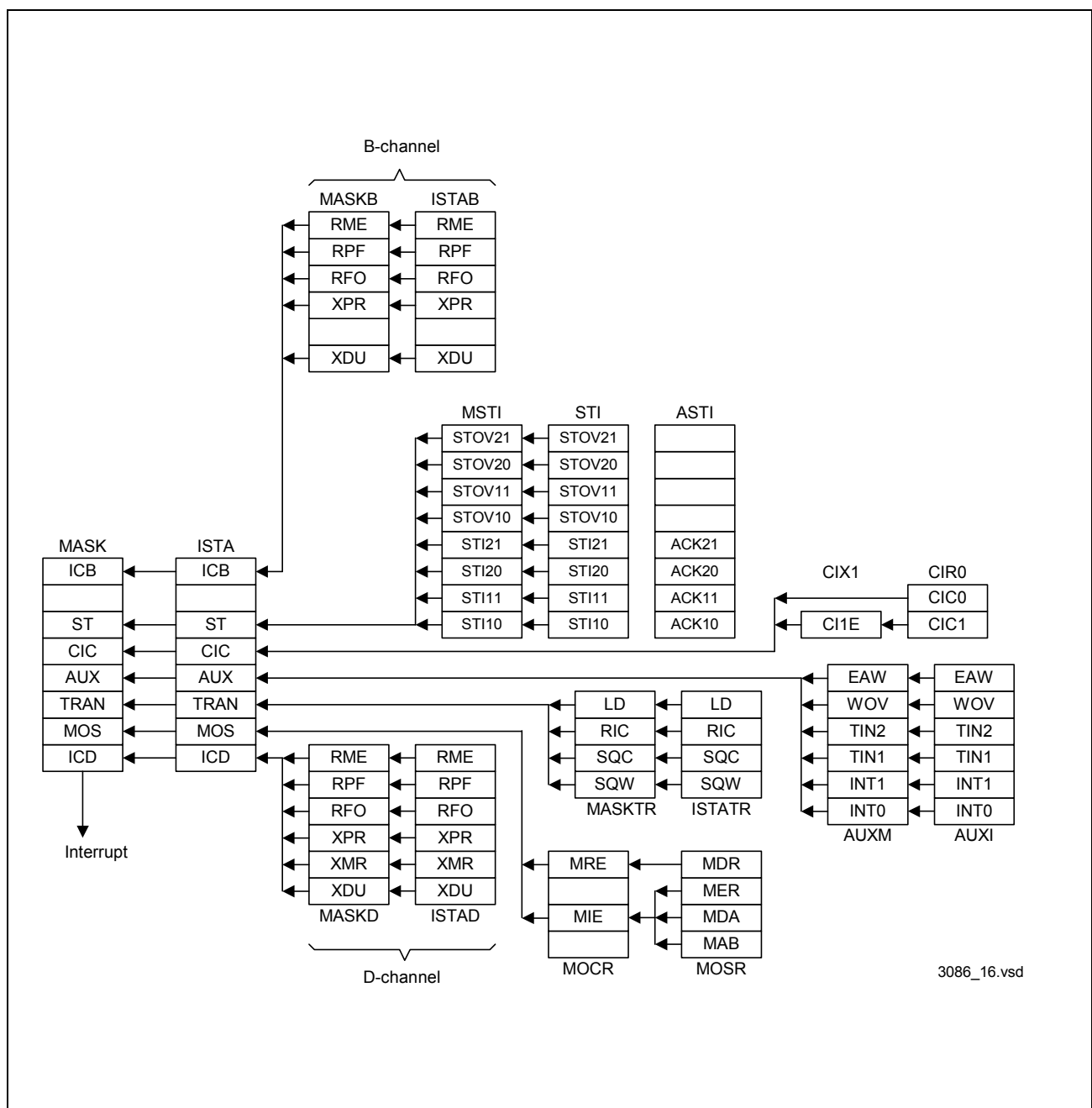
Figure 8 Interrupt Status and Mask Registers
