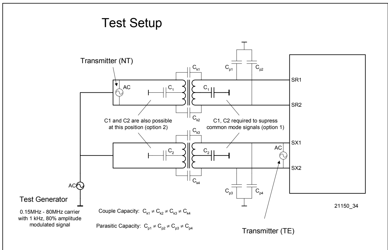
Figure 98 Transformer Circuitry
