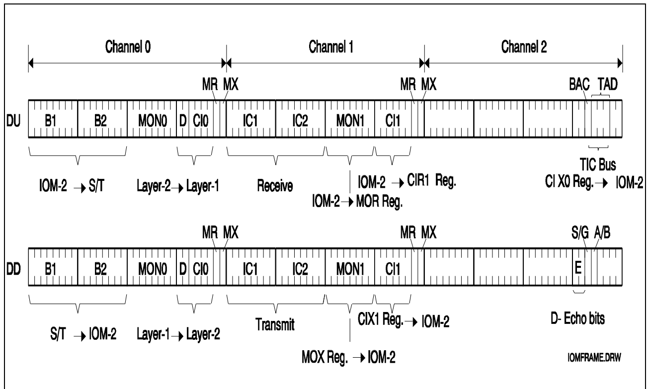
Figure 46 IOM ® -2 Frame Structure in Terminal Mode
