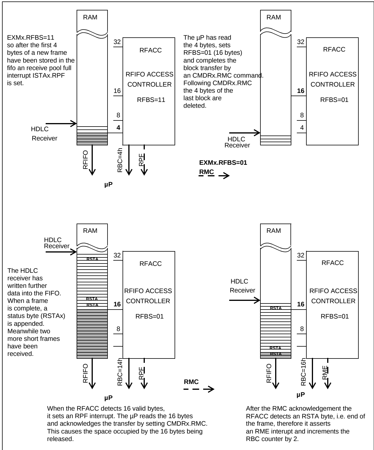
Figure 72 RFIFO Operation
