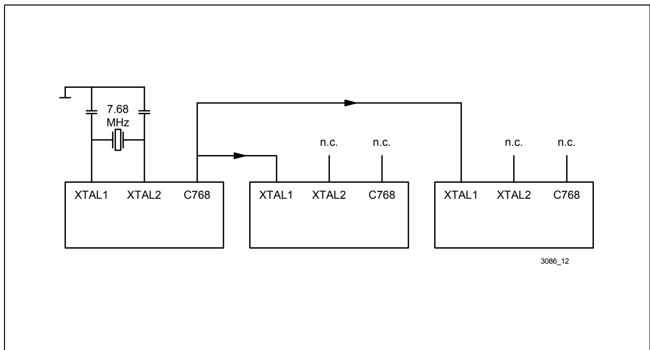
Figure 36 Buffered Oscillator Clock Output
