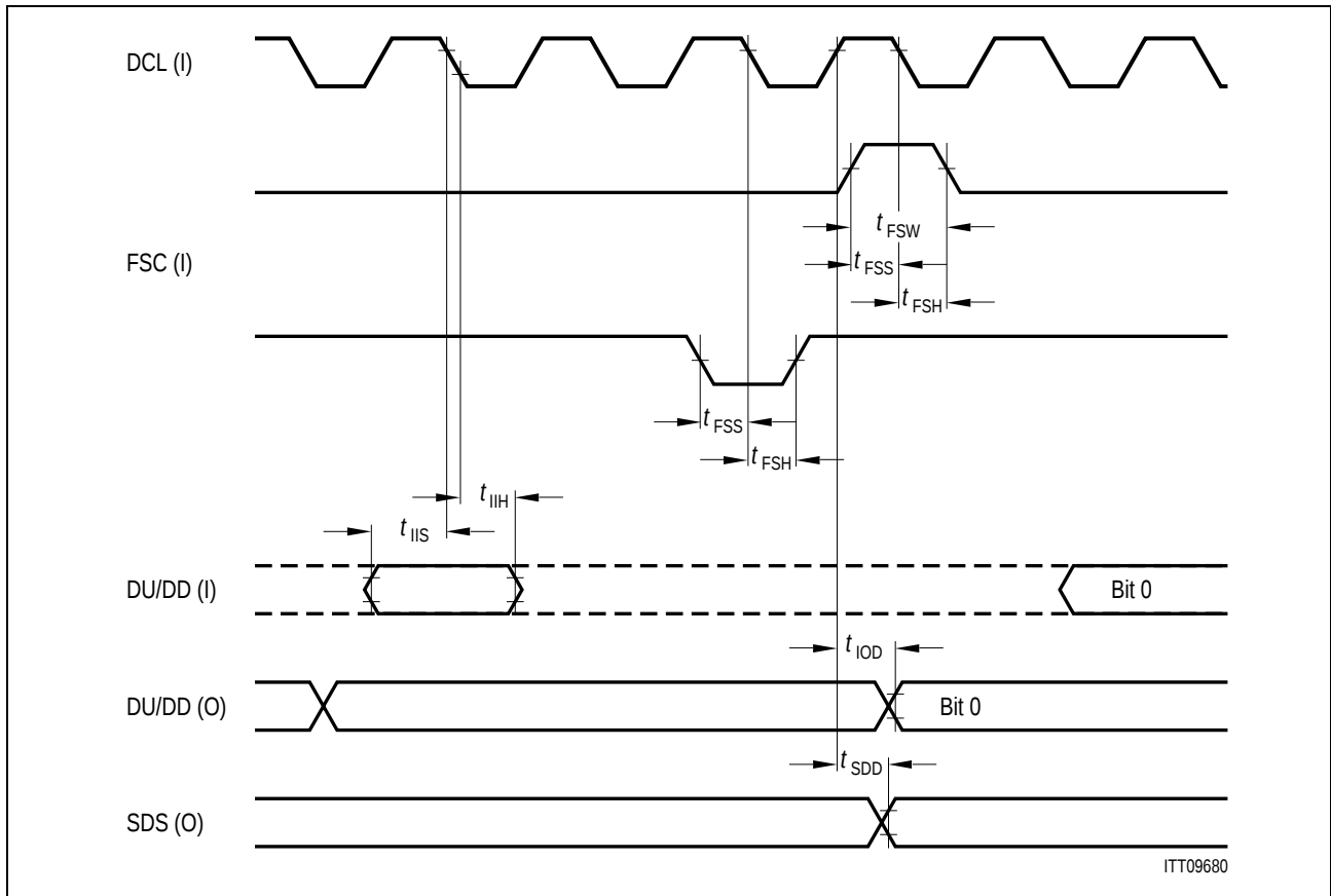
Figure 85 IOM-2 Timing (LT-S, LT-T, NT mode)
