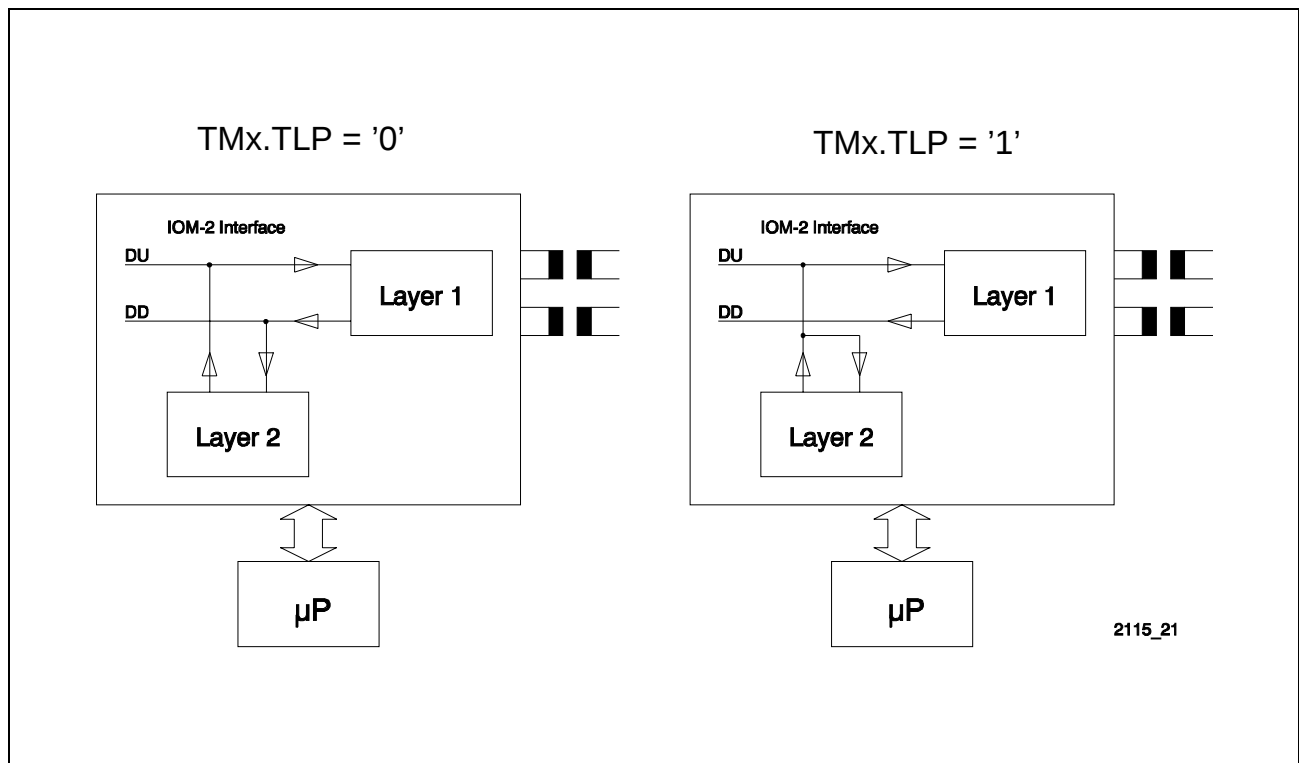
Figure 80 Layer 2 Test Loops
