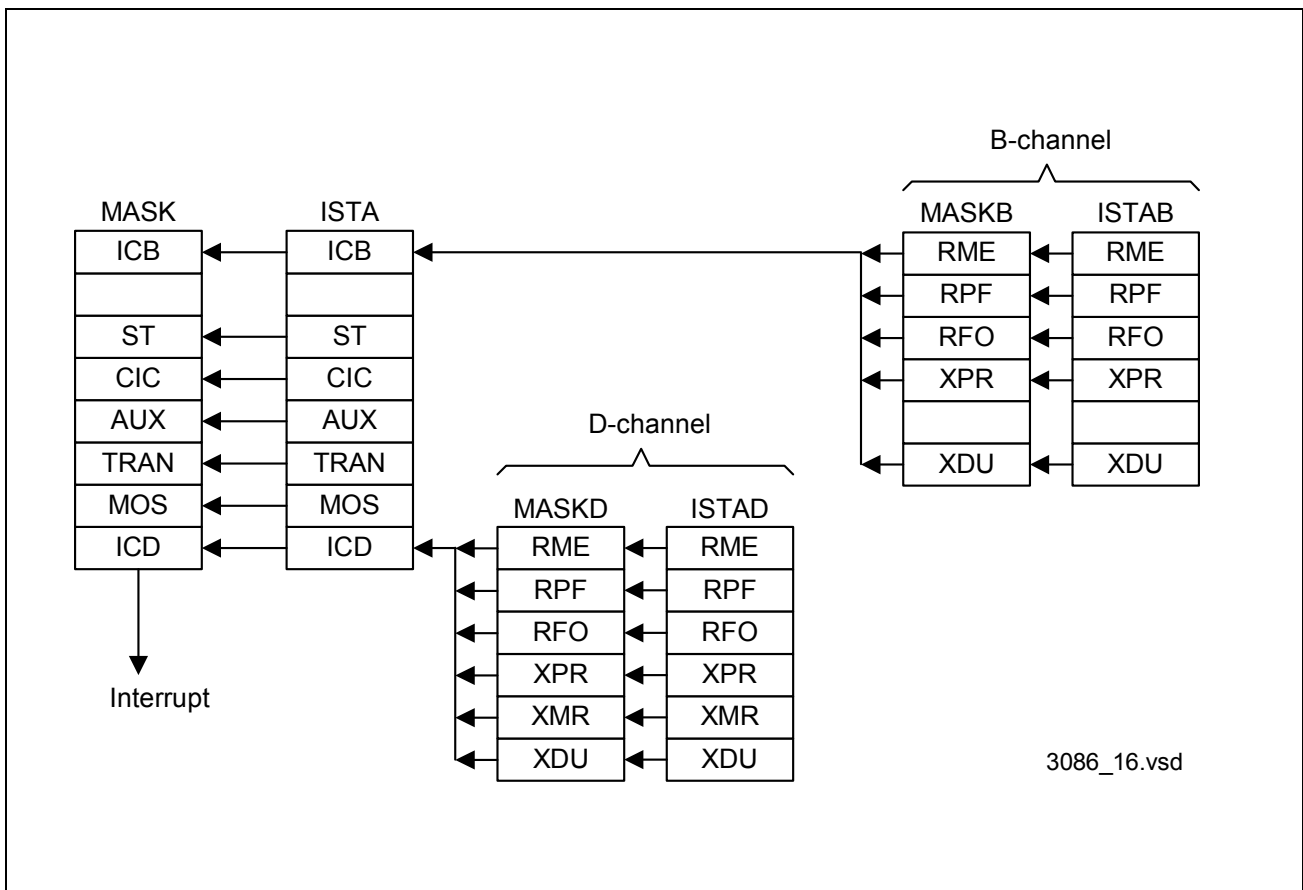
Figure 79 Interrupt Status Registers of the HDLC Controllers
