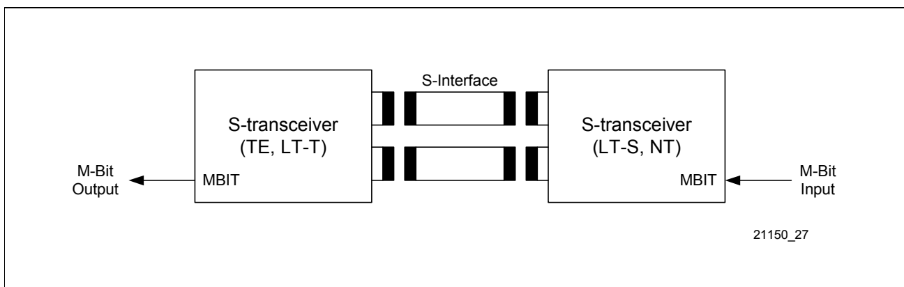
Figure 18 Multiframe Synchronization Using the M-Bit
