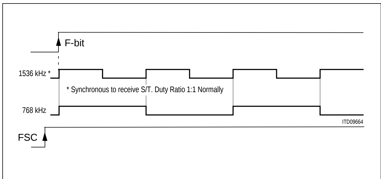
Figure 35 Phase Relationships of ISAC-SX Clock Signals
