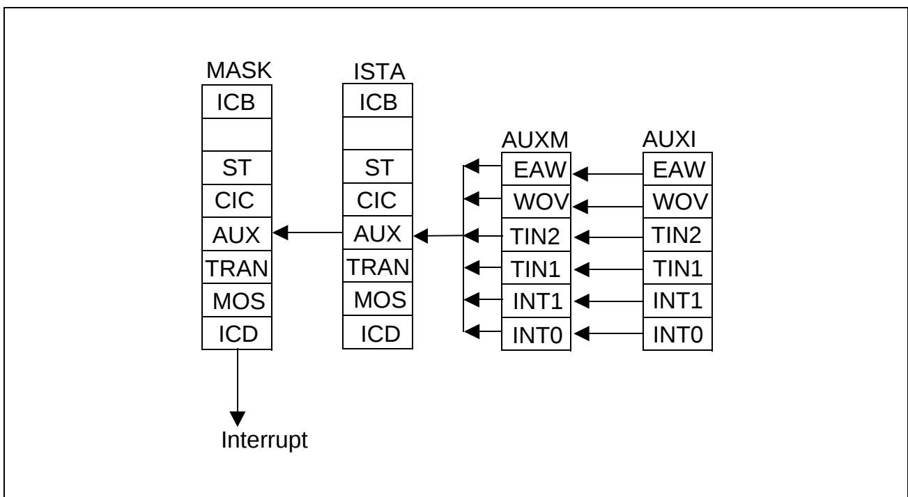
Figure 10 Timer Interrupt Status Registers
