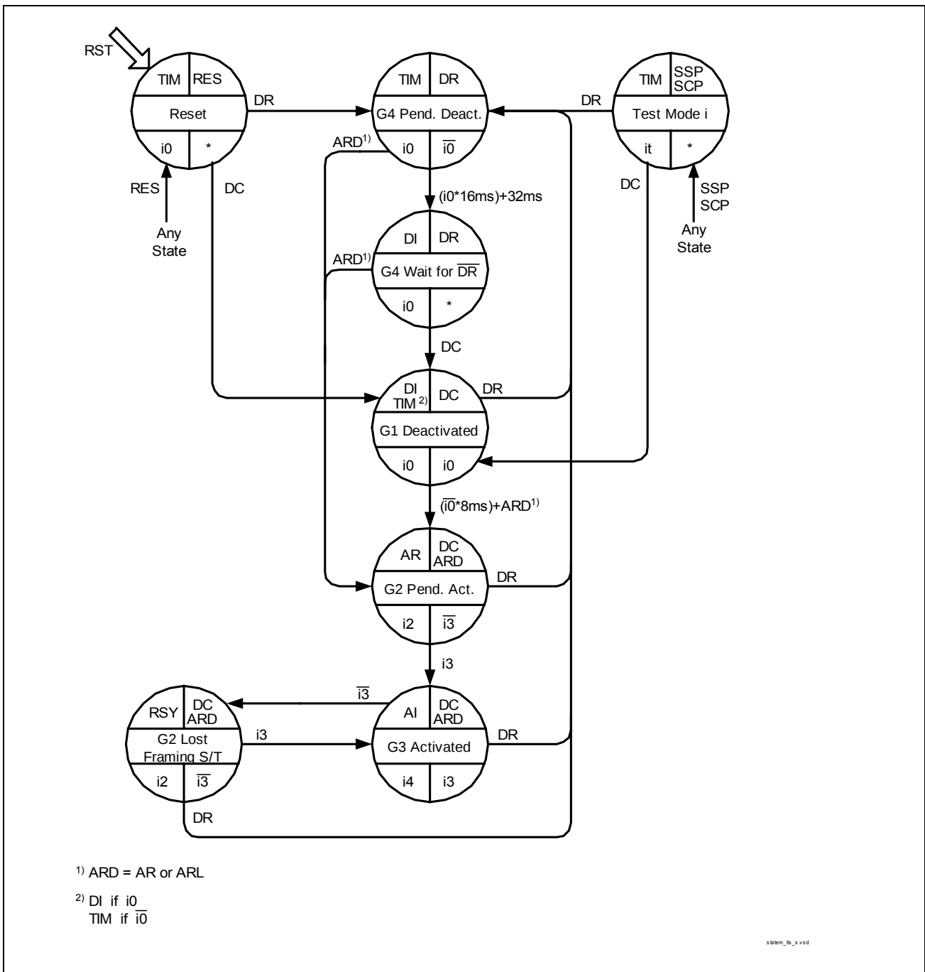
Figure 41 State Transition Diagram (LT-S)
