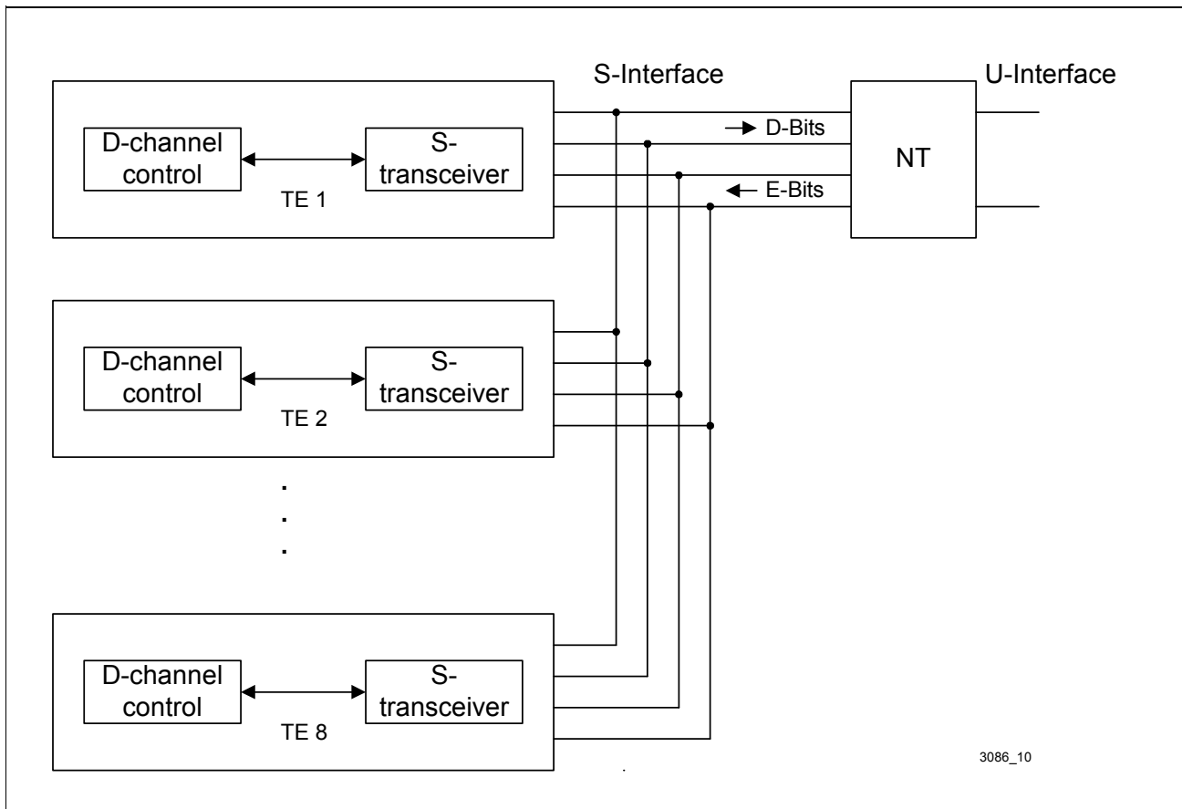
Figure 68 D-Channel Access Control on the S-Interface
