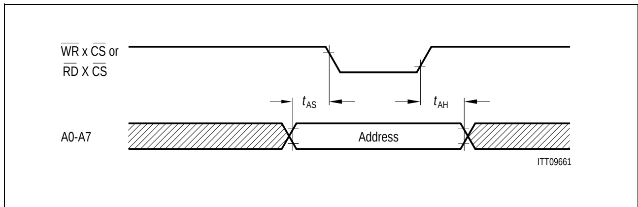
Figure 91 Non-Multiplexed Address Timing
