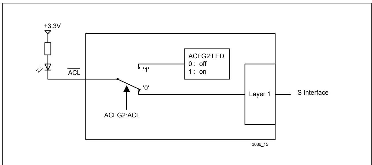
Figure 14 \overline{ACL} Configuration
