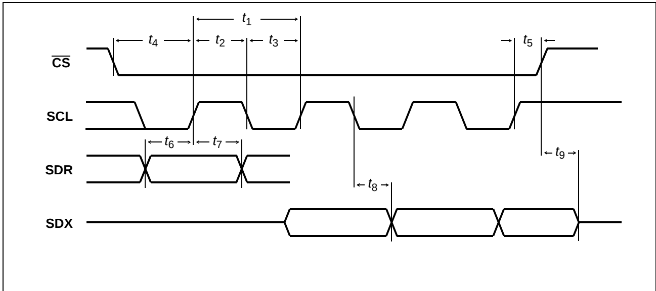
Figure 87 SCI Interface
